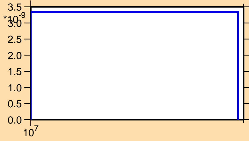
\sigma vs. E for ^{213}\text{Pb}(n,p\alpha)
