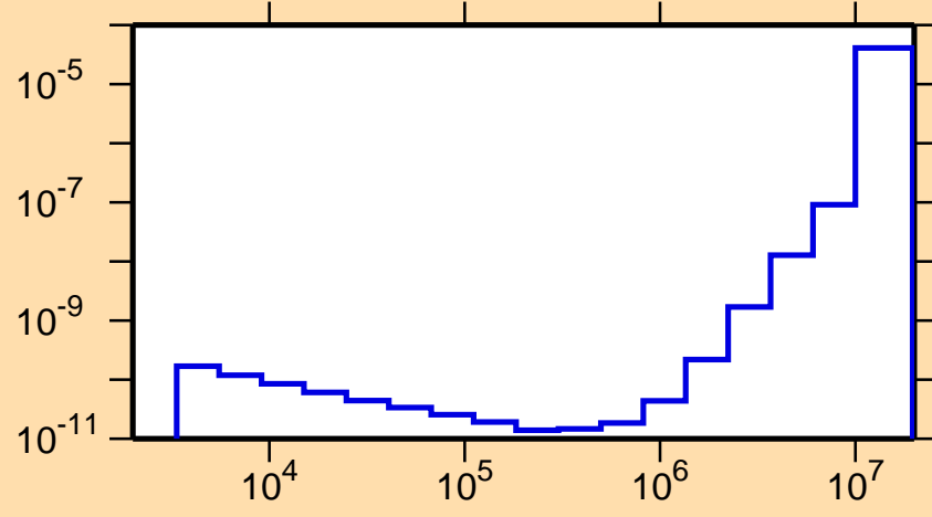
\sigma vs. E for ^{213}\text{Pb}(n,\alpha)
