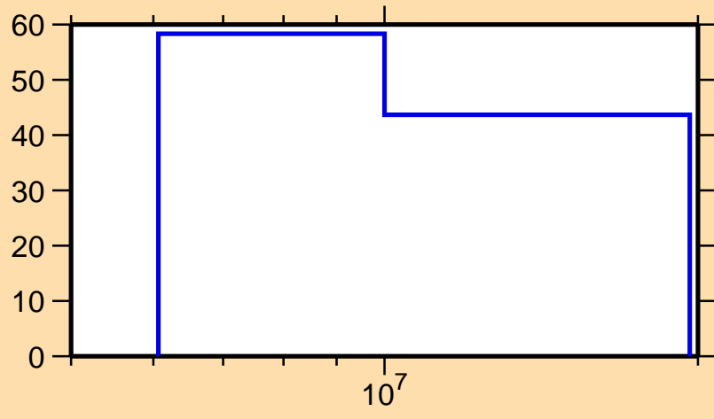
\Delta\sigma/\sigma vs. E for ^{213}\text{Pb}(n,p)
