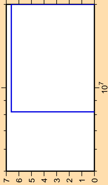
\Delta\sigma/\sigma vs. E for ^{213}\text{Pb}(n,3n)
