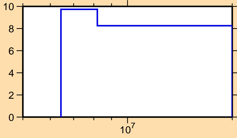
\Delta\sigma/\sigma vs. E for ^{213}\text{Pb}(n,\text{nonel.})
