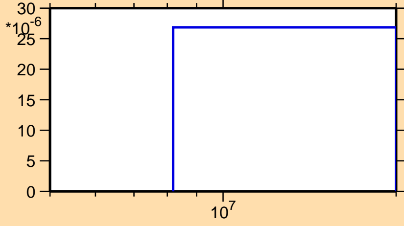
\sigma vs. E for ^{213}\text{Pb}(n,t)
