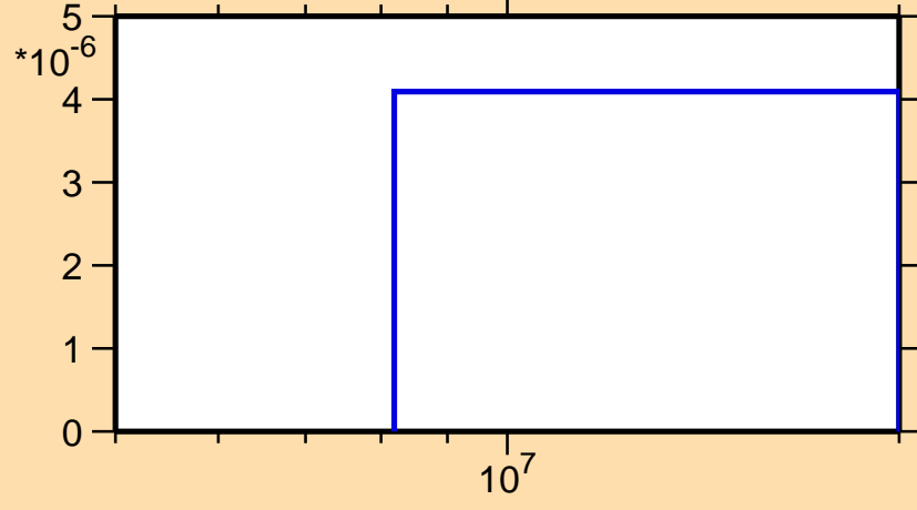
\sigma vs. E for ^{213}\text{Pb}(n,np)
