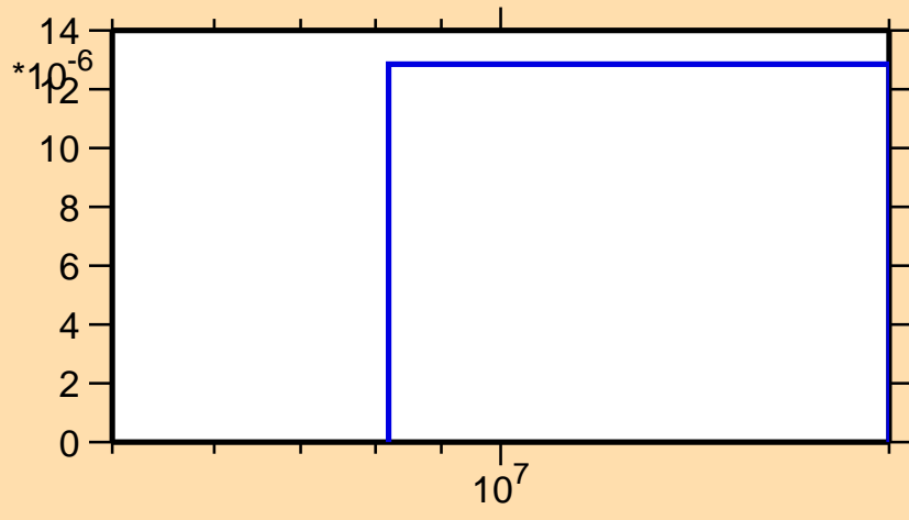
\sigma vs. E for ^{213}\text{Pb}(n,d)
