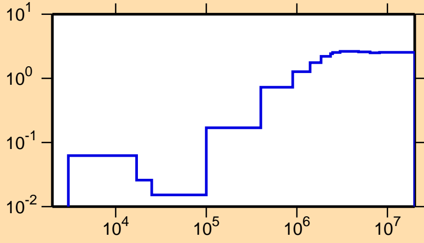
\sigma vs. E for ^{213}\text{Pb}(n,\text{nonel.})
