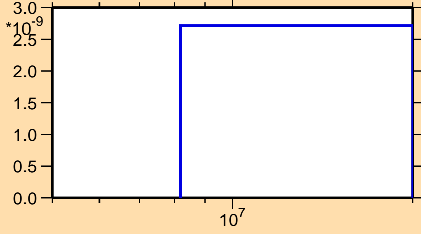
\sigma vs. E for ^{213}\text{Pb}(n,p\alpha)
