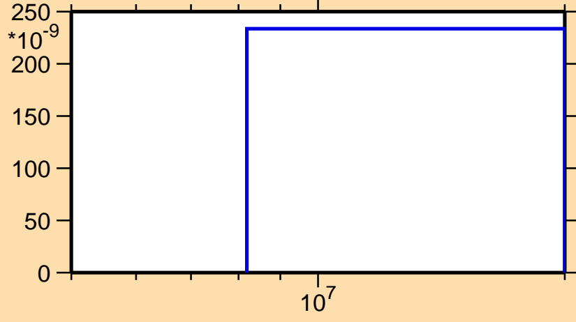
\sigma vs. E for ^{213}\text{Pb}(n,nt)
