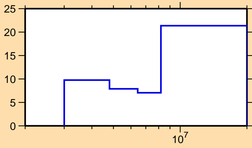
\Delta\sigma/\sigma vs. E for ^{213}\text{Pb}(n,2n)
