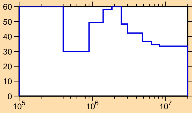
\Delta\sigma/\sigma vs. E for ^{213}\text{Pb}(n,n_1)
