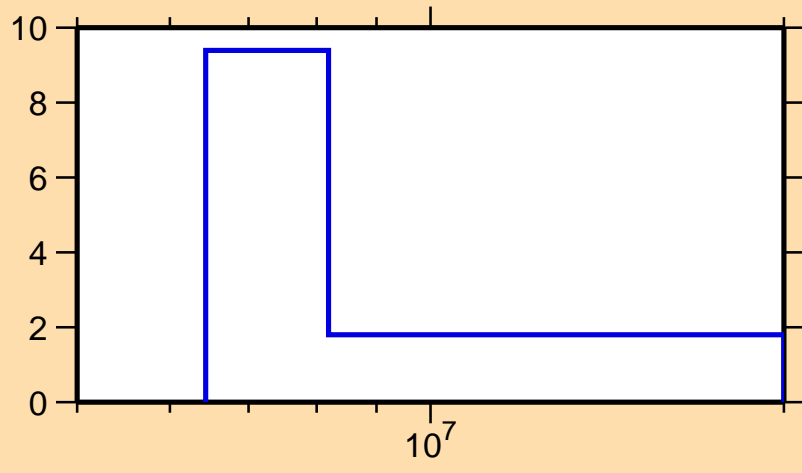
\Delta\sigma/\sigma vs. E for ^{213}\text{Pb}(n,\text{tot.})
