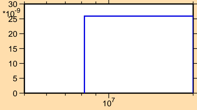
\sigma vs. E for ^{213}\text{Pb}(n,\text{nd})
