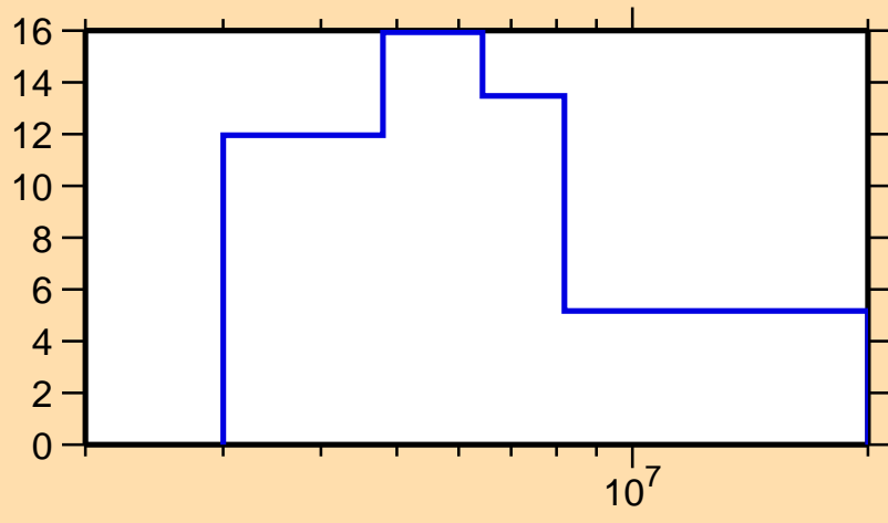
\Delta\sigma/\sigma vs. E for ^{213}\text{Pb}(n,\text{el.})
