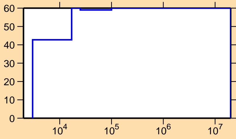
\Delta\sigma/\sigma vs. E for ^{213}\text{Pb}(n,\gamma)
