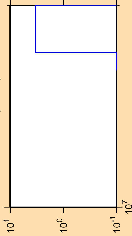
\Delta\sigma/\sigma vs. E for ^{214}\text{Pb} (mt 45)
