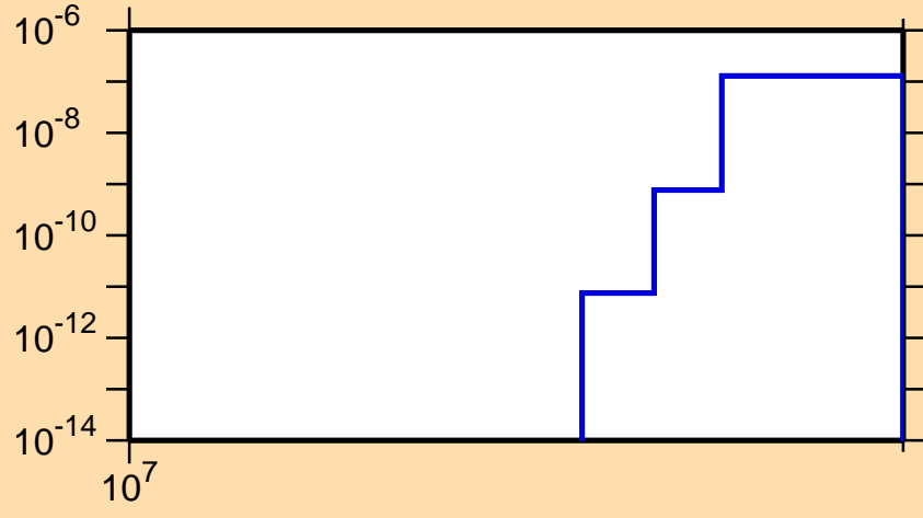
\sigma vs. E for ^{214}\text{Pb}(n,\text{nd})
