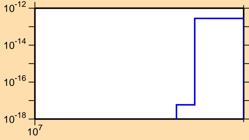
\sigma vs. E for ^{214}\text{Pb} (mt 11)
