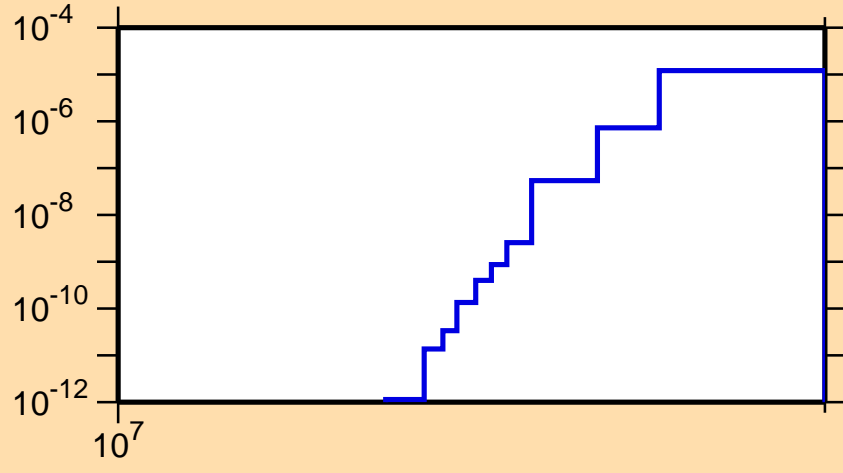
\sigma vs. E for ^{214}\text{Pb}(n,nt)
