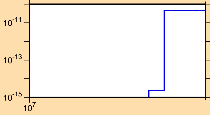
\sigma vs. E for ^{214}\text{Pb}(\text{mt117})
