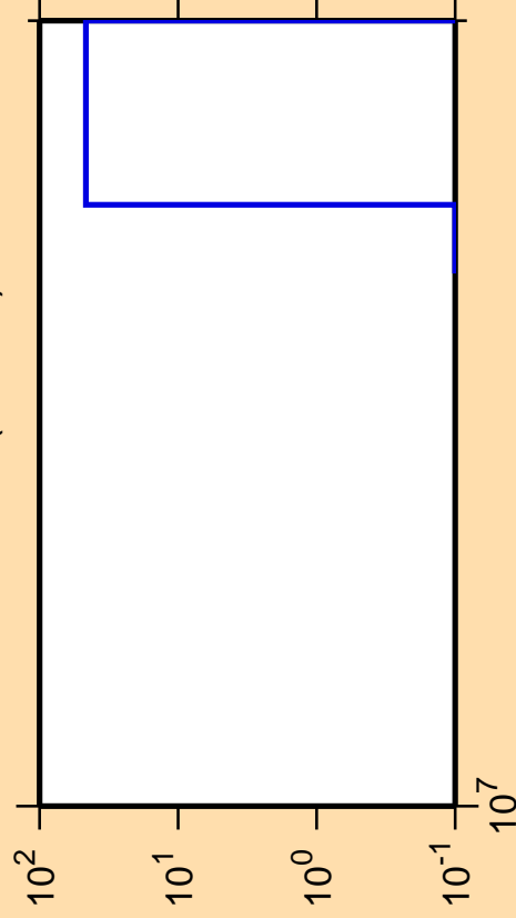
\Delta\sigma/\sigma vs. E for ^{214}\text{Pb}(\text{mt117})
