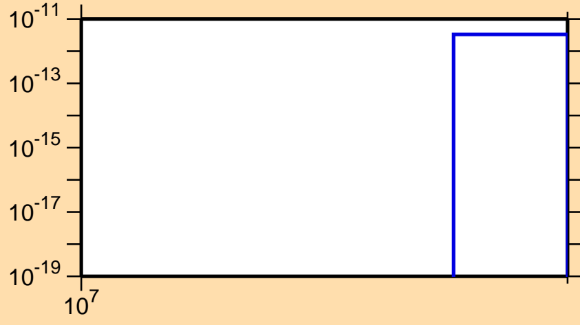
\sigma vs. E for ^{214}\text{Pb} (mt 45)
