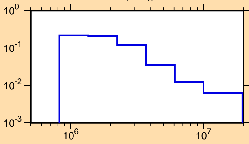
\sigma vs. E for ^{214}\text{Pb}(n,n_1)
