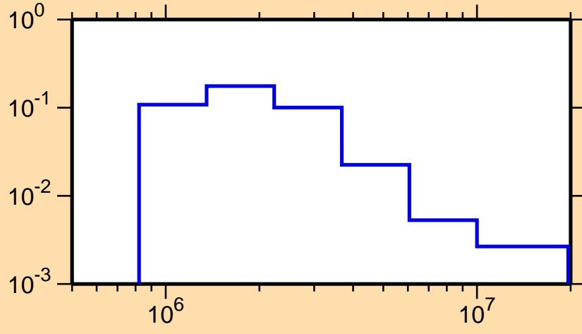
\sigma vs. E for ^{214}\text{Pb}(n,n_2)
