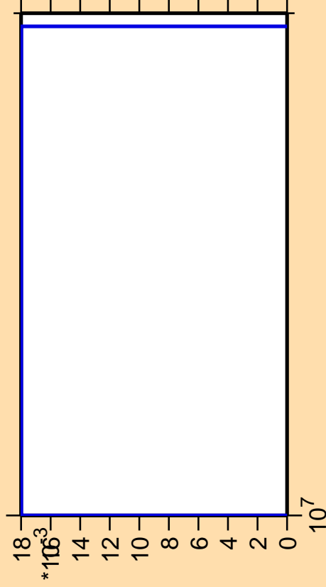
\Delta\sigma/\sigma vs. E for ^{214}\text{Pb} (mt 45)
