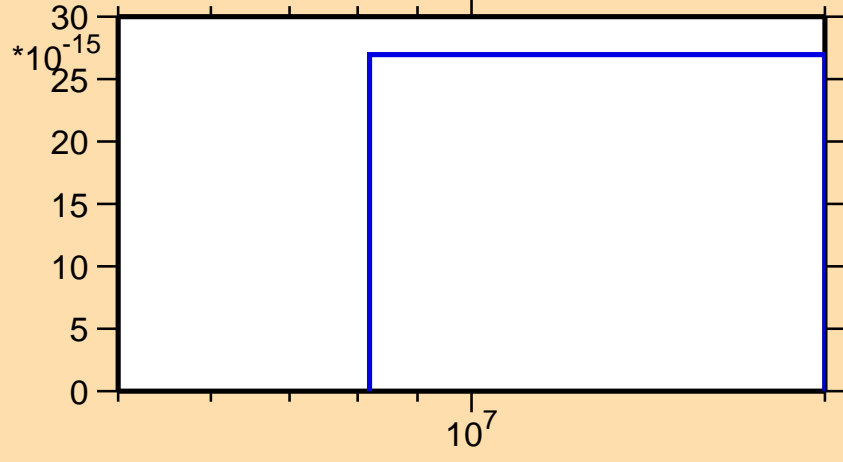
\sigma vs. E for ^{214}\text{Pb}(\text{mt } 45)
