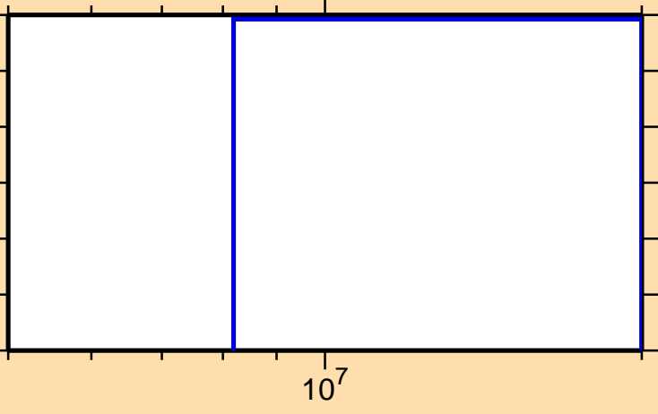
\sigma vs. E for ^{214}\text{Pb}(n,t)
