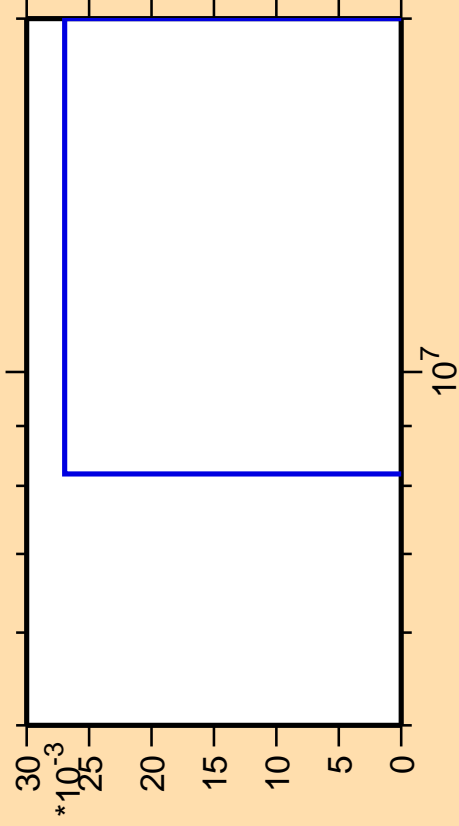
\Delta\sigma/\sigma vs. E for ^{214}\text{Pb}(\text{mt } 45)
