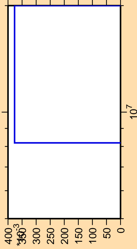
\Delta\sigma/\sigma vs. E for ^{214}\text{Pb}(\text{mt117})
