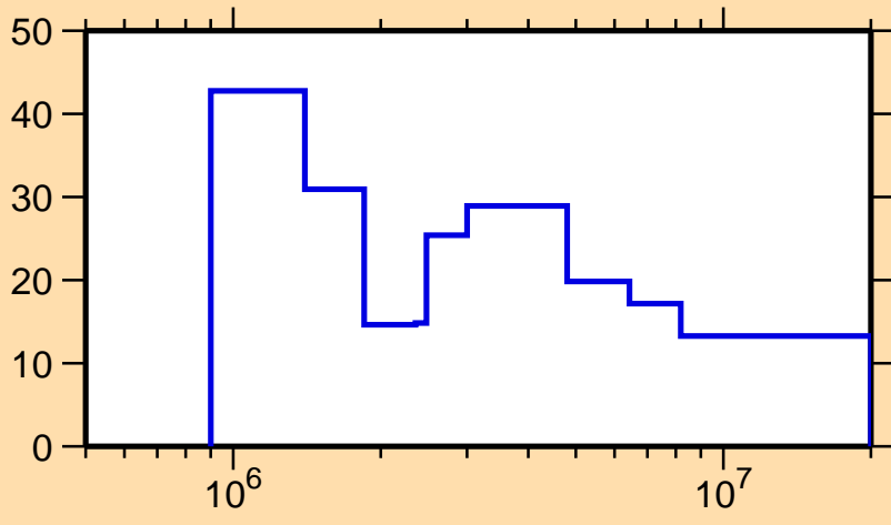
\Delta\sigma/\sigma vs. E for ^{214}\text{Pb}(n, tot.)
