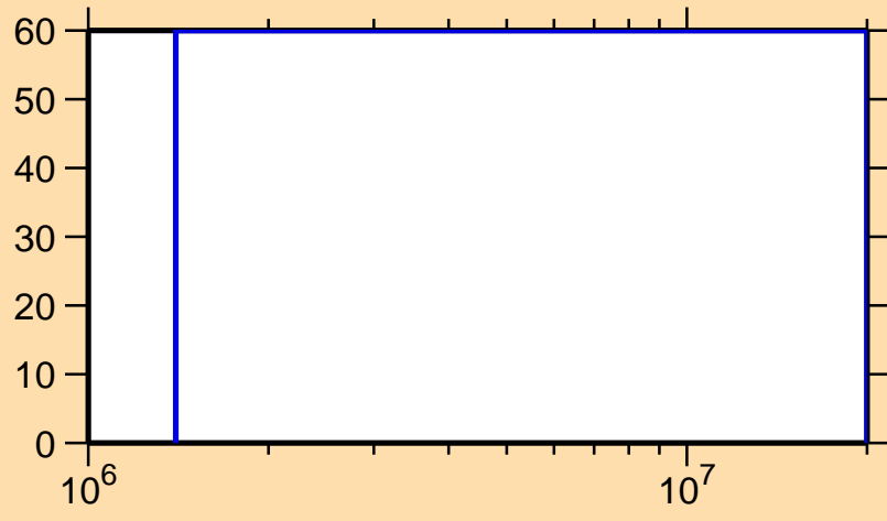
\Delta\sigma/\sigma vs. E for ^{214}\text{Pb}(n,\gamma)
