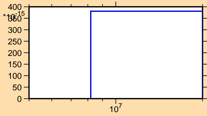
\sigma vs. E for ^{214}\text{Pb}(\text{mt117})
