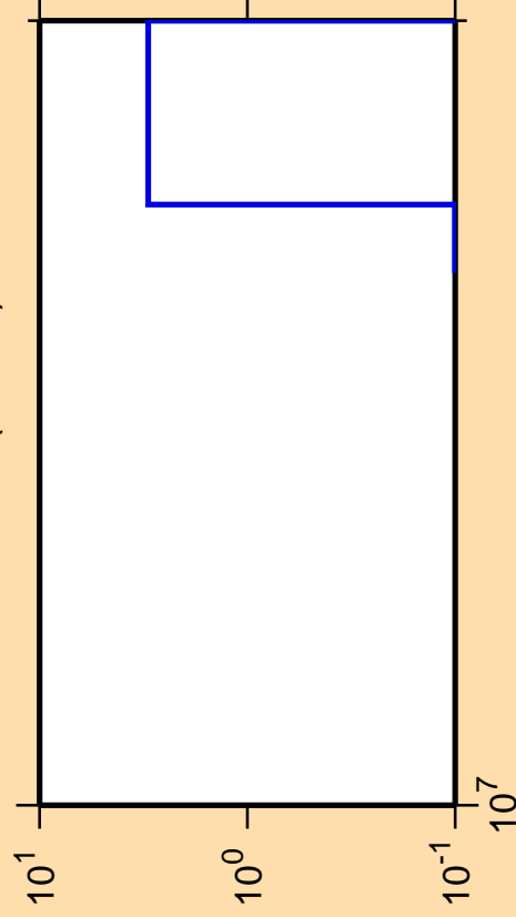
\Delta\sigma/\sigma vs. E for ^{215}\text{Pb} (mt 11)
