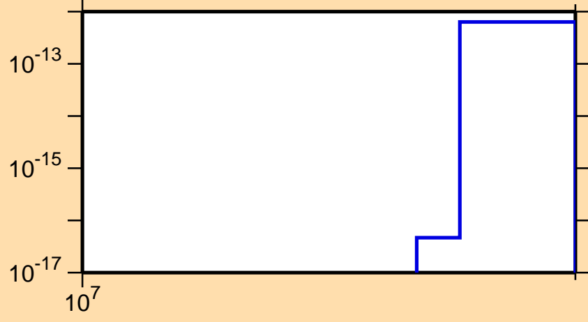
\sigma vs. E for ^{215}\text{Pb} (mt 11)
