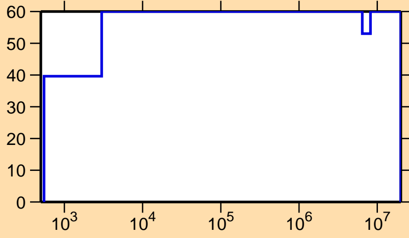
\Delta\sigma/\sigma vs. E for ^{215}\text{Pb}(n,\gamma)
