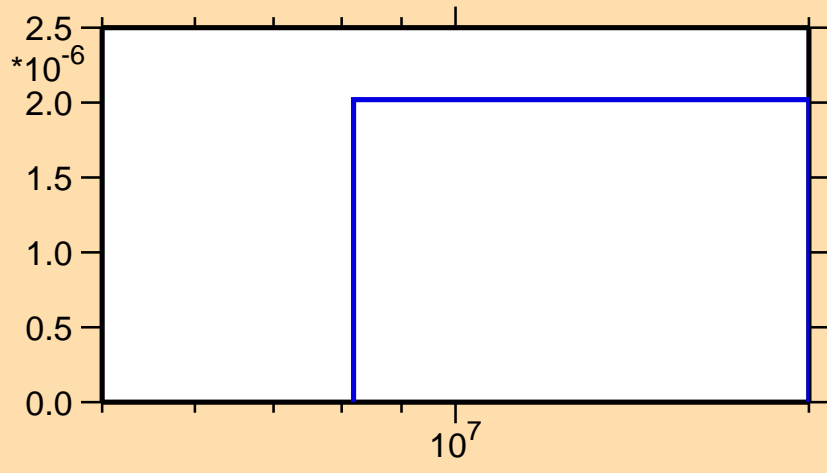
\sigma vs. E for ^{215}\text{Pb}(n,np)
