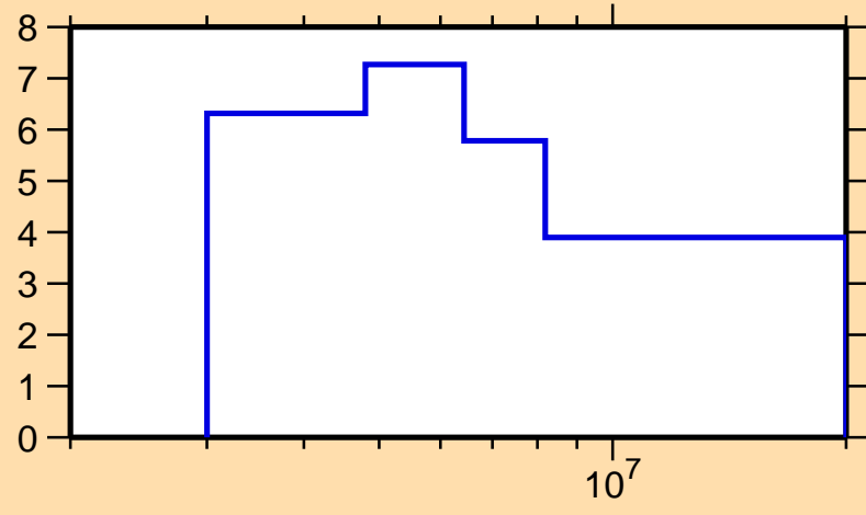
\Delta\sigma/\sigma vs. E for ^{215}\text{Pb}(n,\text{tot.})
