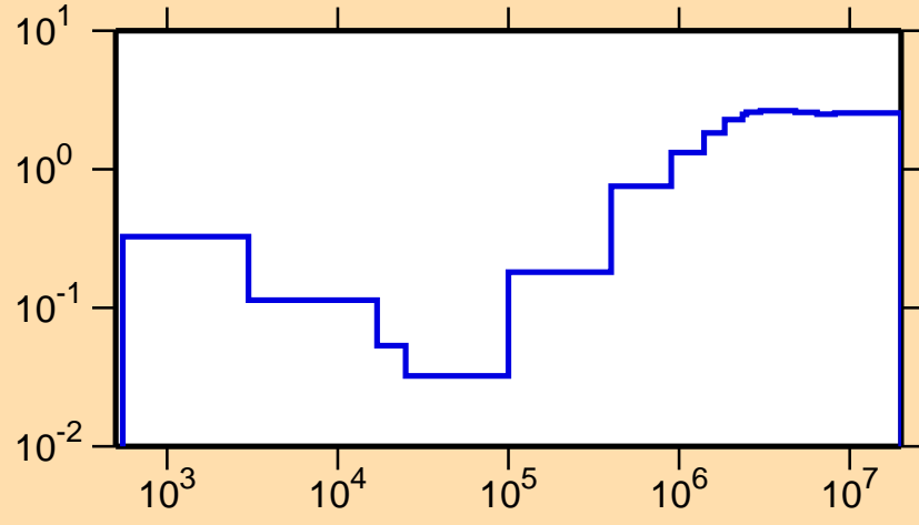
\sigma vs. E for ^{215}\text{Pb}(n,\text{nonel.})
