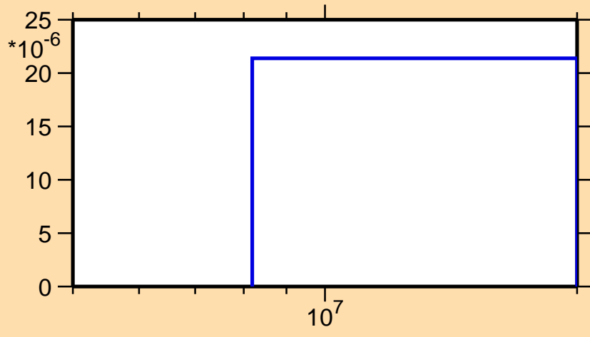
\sigma vs. E for ^{215}\text{Pb}(n,t)
