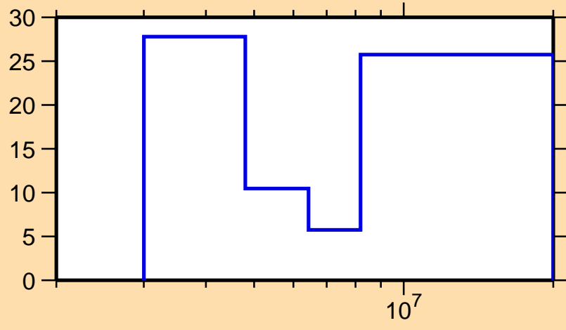
\Delta\sigma/\sigma vs. E for ^{215}\text{Pb}(n,2n)
