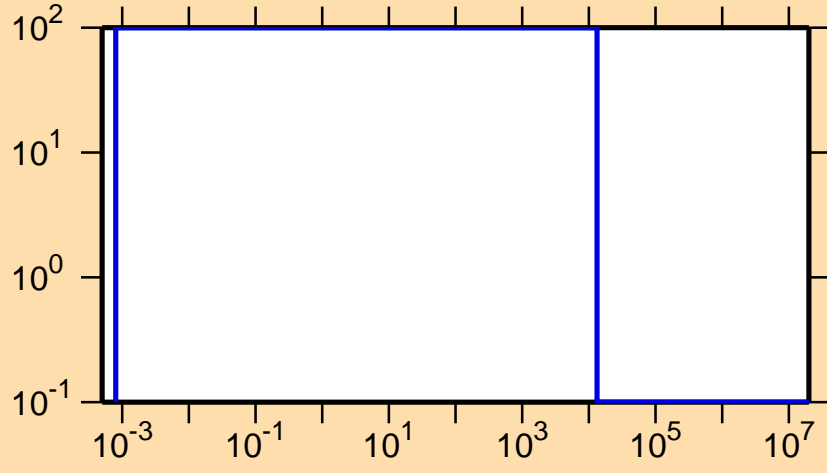
\Delta\sigma/\sigma vs. E for ^{216}\text{Pb}(n,f)
