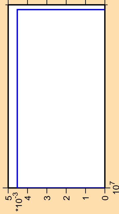
\Delta\sigma/\sigma vs. E for ^{216}\text{Pb} (mt 11)
