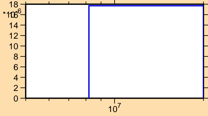
\sigma vs. E for ^{216}\text{Pb}(n,p)
