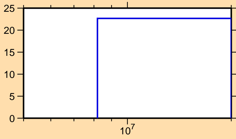
\Delta\sigma/\sigma vs. E for ^{216}\text{Pb}(n,\text{tot.})
