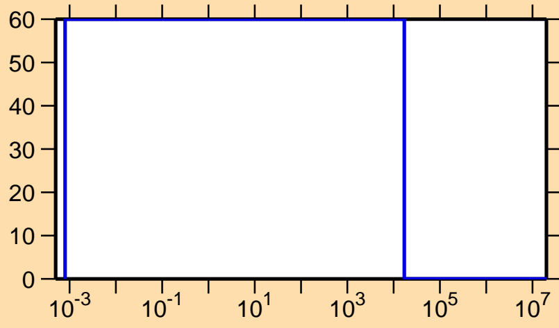
\Delta\sigma/\sigma vs. E for ^{216}\text{Pb}(n,f)
