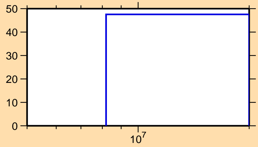
\Delta\sigma/\sigma vs. E for ^{216}\text{Pb}(n,el.)
