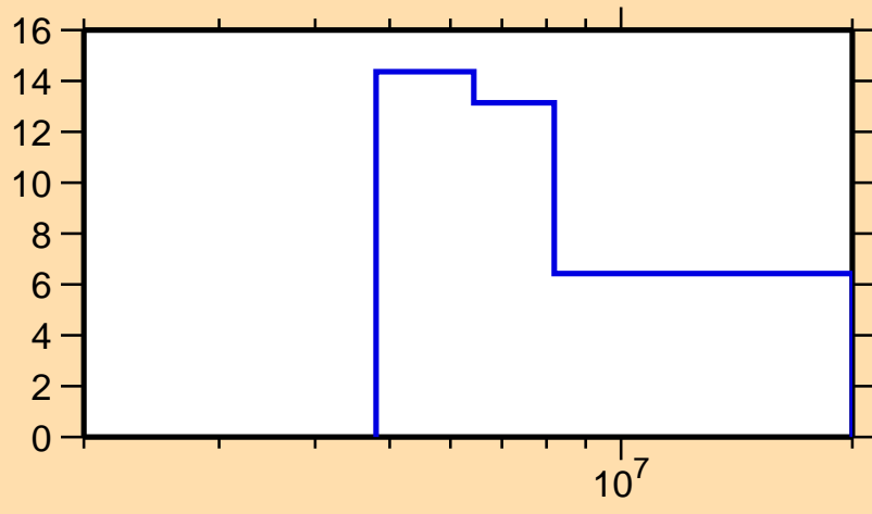
\Delta\sigma/\sigma vs. E for ^{216}\text{Pb}(n,\text{nonel.})
