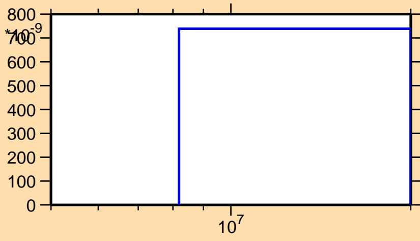
\sigma vs. E for ^{216}\text{Pb}(n,np)
