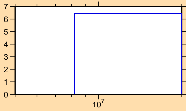
\Delta\sigma/\sigma vs. E for ^{216}\text{Pb}(n,\text{nonel.})
