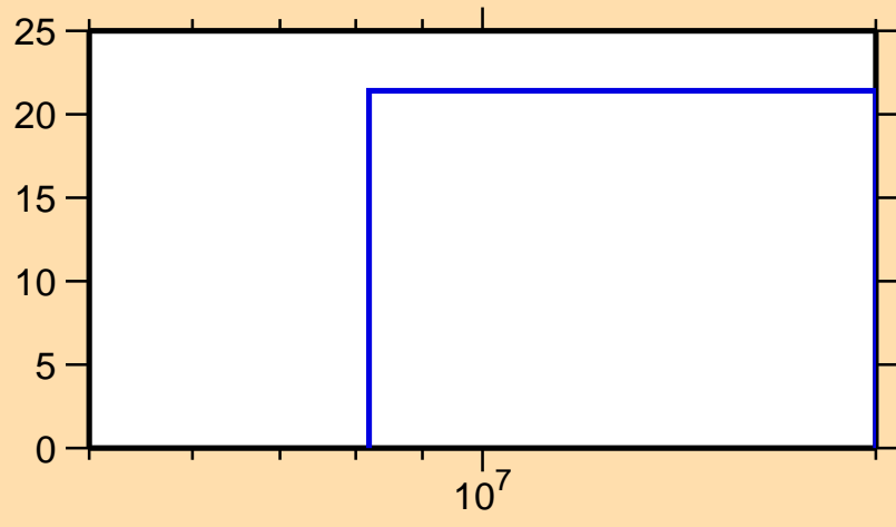
\Delta\sigma/\sigma vs. E for ^{216}\text{Pb}(n,2n)
