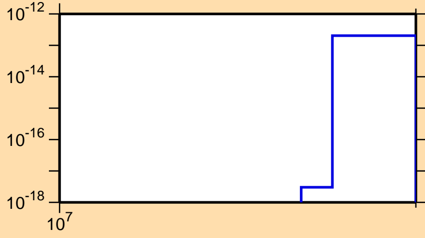
\sigma vs. E for ^{217}\text{Pb} (mt 11)
