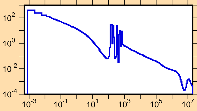
\sigma vs. E for ^{217}\text{Pb}(n,\gamma)
