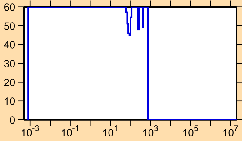
\Delta\sigma/\sigma vs. E for ^{217}\text{Pb}(n,f)
