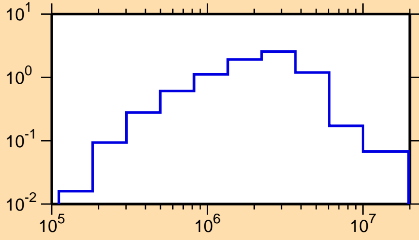
\sigma vs. E for ^{217}\text{Pb}(n,n\text{cont.})
