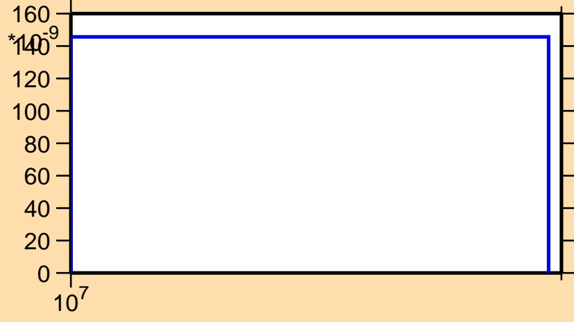
\sigma vs. E for ^{217}\text{Pb}(n,nt)
