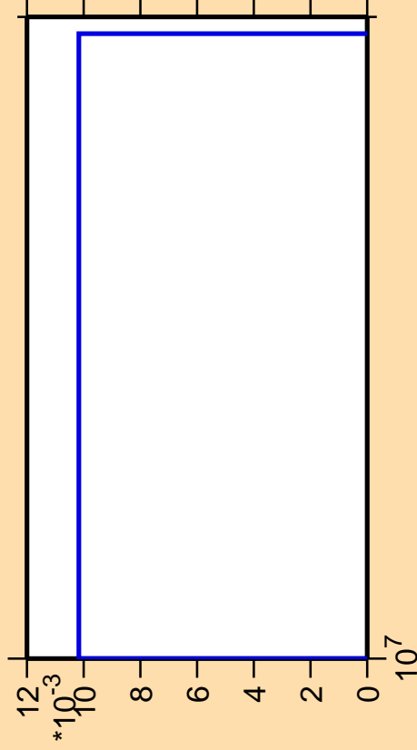
\Delta\sigma/\sigma vs. E for ^{217}\text{Pb} (mt 11)
