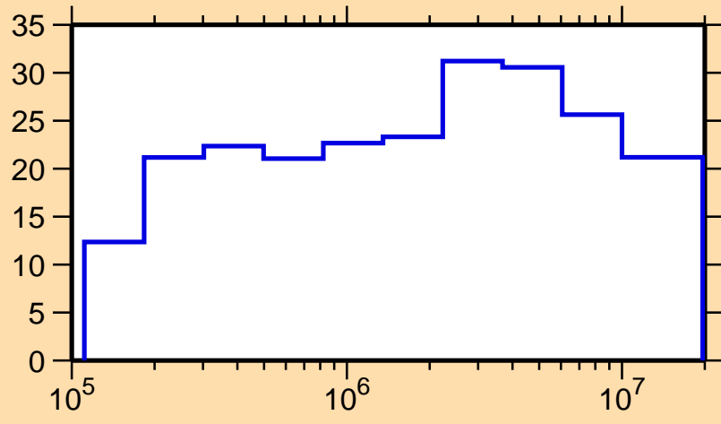
\Delta\sigma/\sigma vs. E for ^{217}\text{Pb}(n,\text{nonel.})
