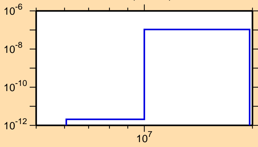
\sigma vs. E for ^{217}\text{Pb}(n,2n\alpha)
