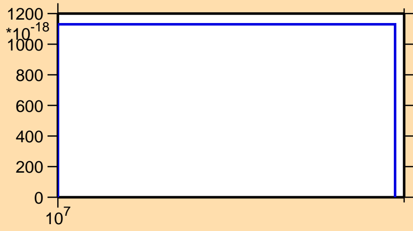
\sigma vs. E for ^{217}\text{Pb} (mt 11)
