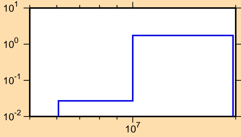
\sigma vs. E for ^{217}\text{Pb}(n,3n)
