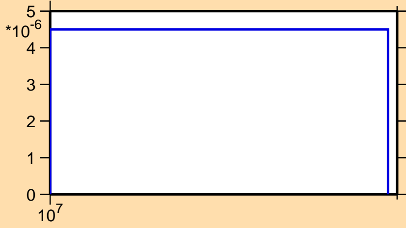
\sigma vs. E for ^{217}\text{Pb}(n,d)
