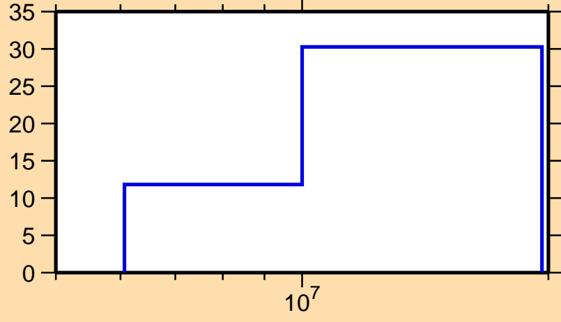
\Delta\sigma/\sigma vs. E for ^{217}\text{Pb}(n,p)
