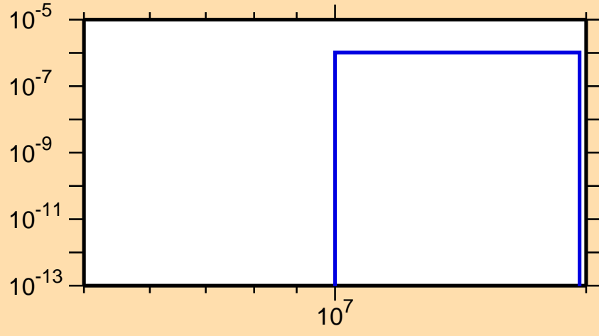
\sigma vs. E for ^{217}\text{Pb}(n,np)
