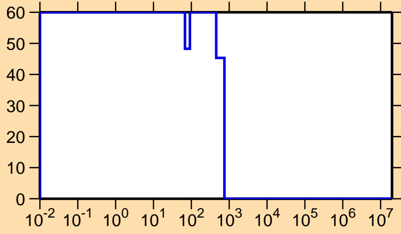
\Delta\sigma/\sigma vs. E for ^{217}\text{Pb}(n,f)
