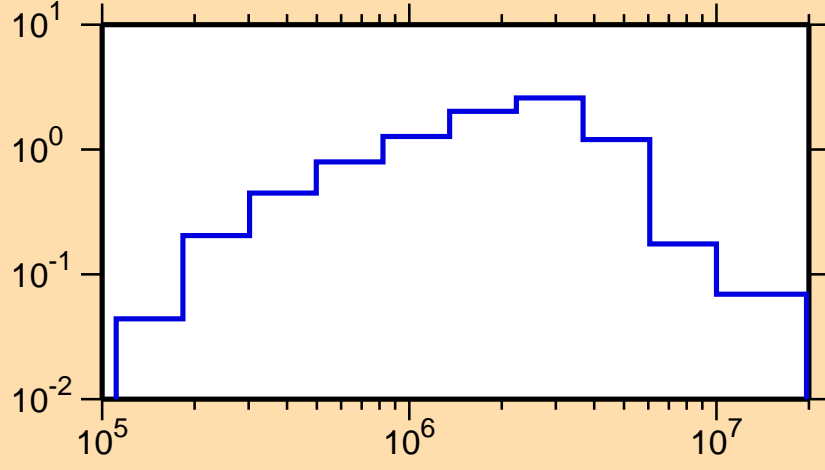
\sigma vs. E for ^{217}\text{Pb}(n,\text{inel.})
