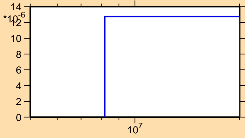
\sigma vs. E for ^{217}\text{Pb}(n,t)
