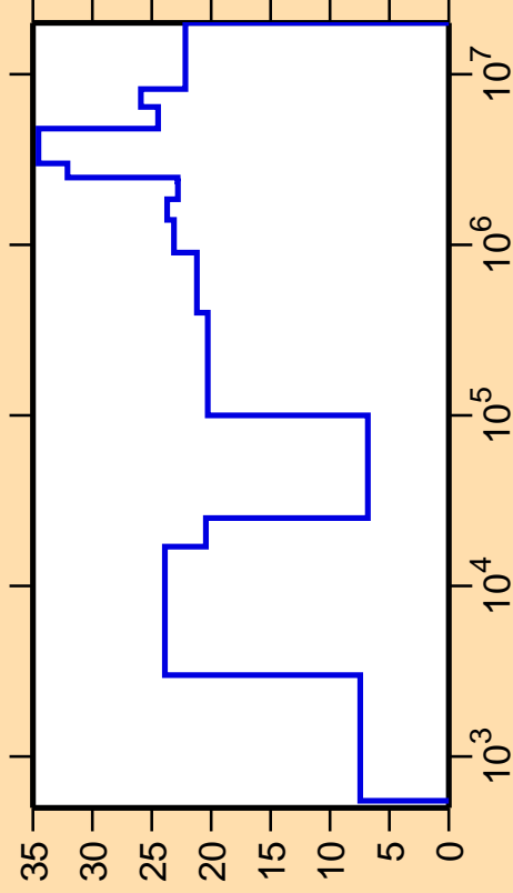
\Delta\sigma/\sigma vs. E for ^{217}\text{Pb}(n,\text{nonel.})
