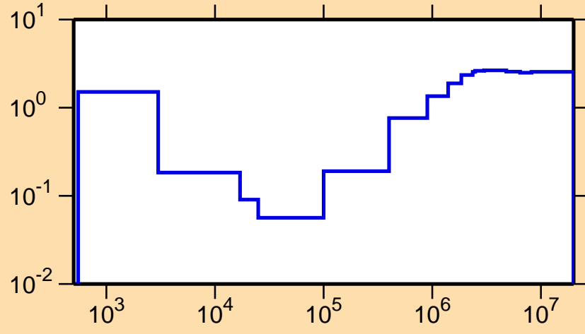
\sigma vs. E for ^{217}\text{Pb}(n,\text{nonel.})
