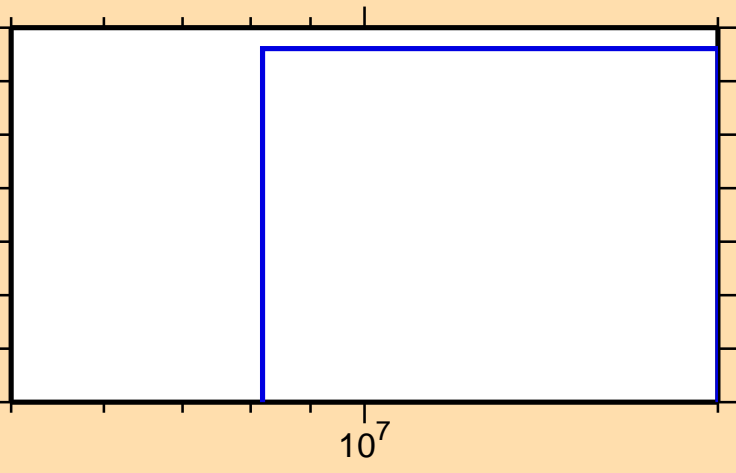
\sigma vs. E for ^{217}\text{Pb}(n,\text{nd})
