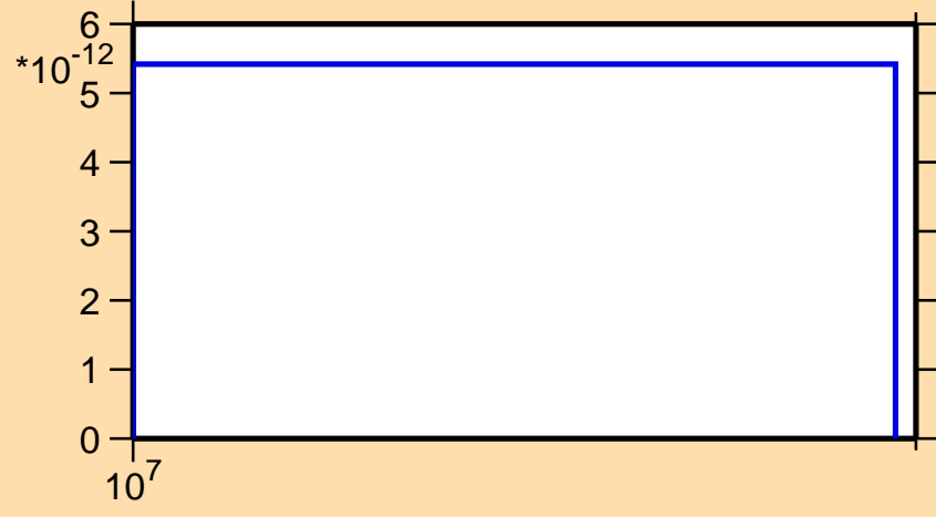
\sigma vs. E for ^{218}\text{Pb}(n,2np)
