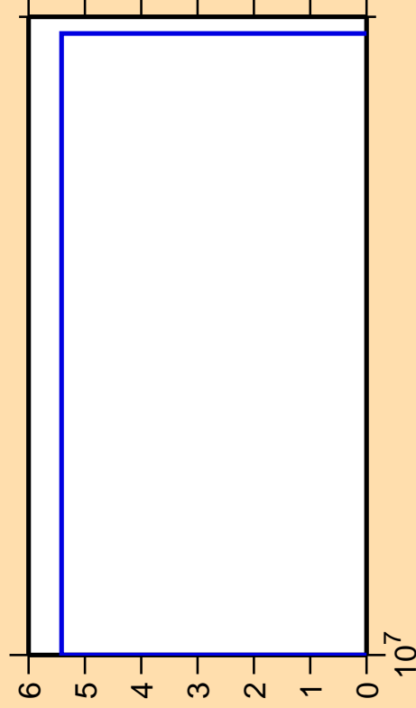
\Delta\sigma/\sigma vs. E for ^{218}\text{Pb}(n,2np)
