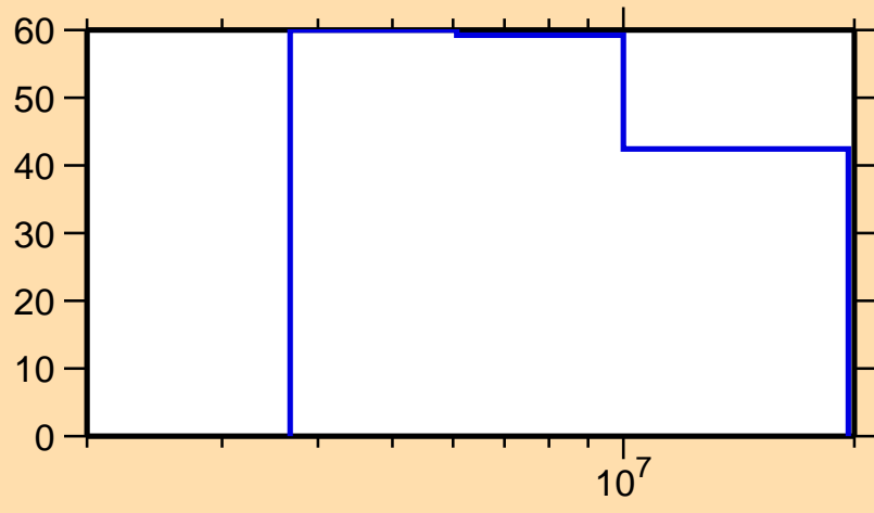
\Delta\sigma/\sigma vs. E for ^{218}\text{Pb}(n,\text{nonel.})
