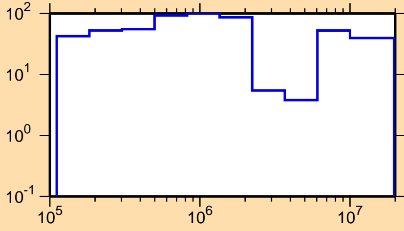
\Delta\sigma/\sigma vs. E for ^{218}\text{Pb}(n,\text{el.})
