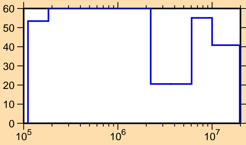
\Delta\sigma/\sigma vs. E for ^{218}\text{Pb}(n,\text{tot.})
