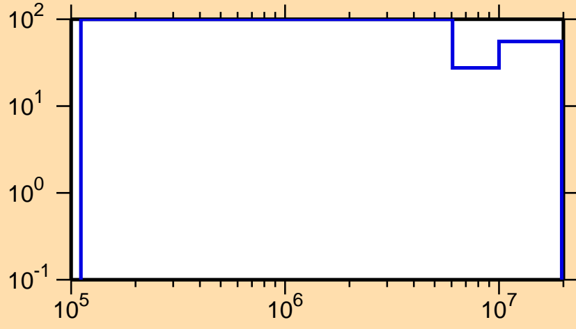
\Delta\sigma/\sigma vs. E for ^{218}\text{Pb}(n,n_1)
