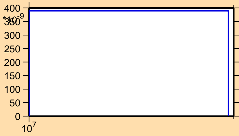
\sigma vs. E for ^{218}\text{Pb}(n,np)
