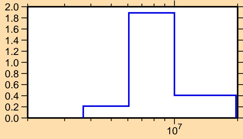
\sigma vs. E for ^{218}\text{Pb}(n,2n)
