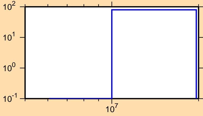
\Delta\sigma/\sigma vs. E for ^{218}\text{Pb}(n,p)
