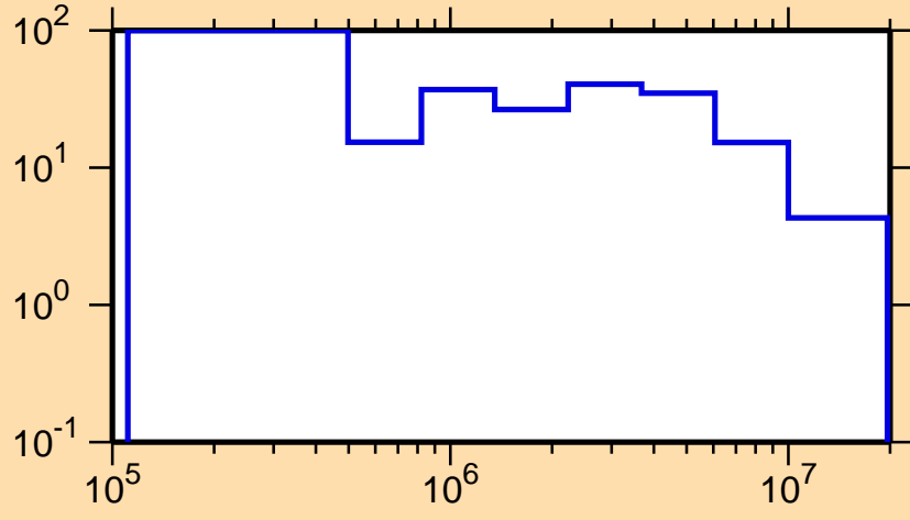
\Delta\sigma/\sigma vs. E for ^{218}\text{Pb}(n,n\text{cont.})
