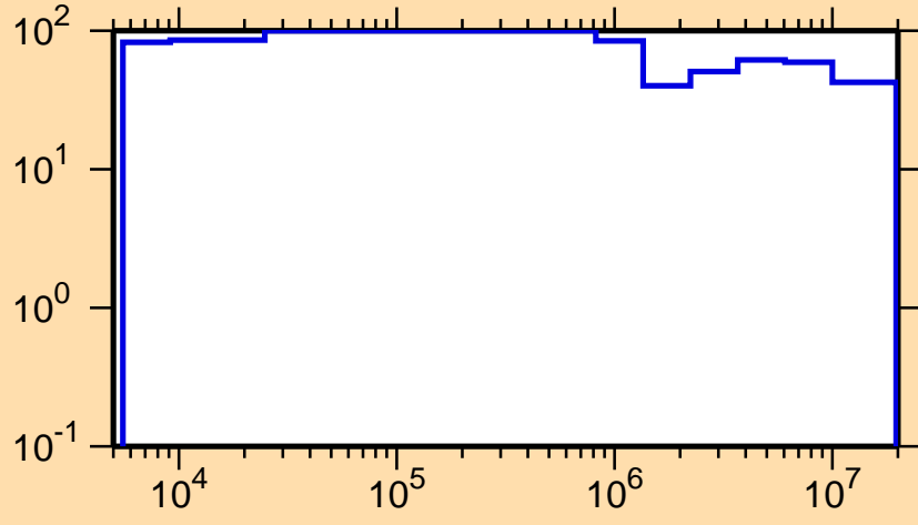
\Delta\sigma/\sigma vs. E for ^{218}\text{Pb}(n,\text{nonel.})
