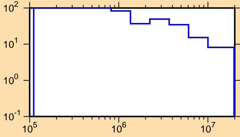
\Delta\sigma/\sigma vs. E for ^{218}\text{Pb}(n,\text{inel.})
