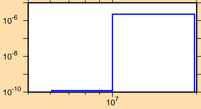
\sigma vs. E for ^{218}\text{Pb}(n,n\alpha)
