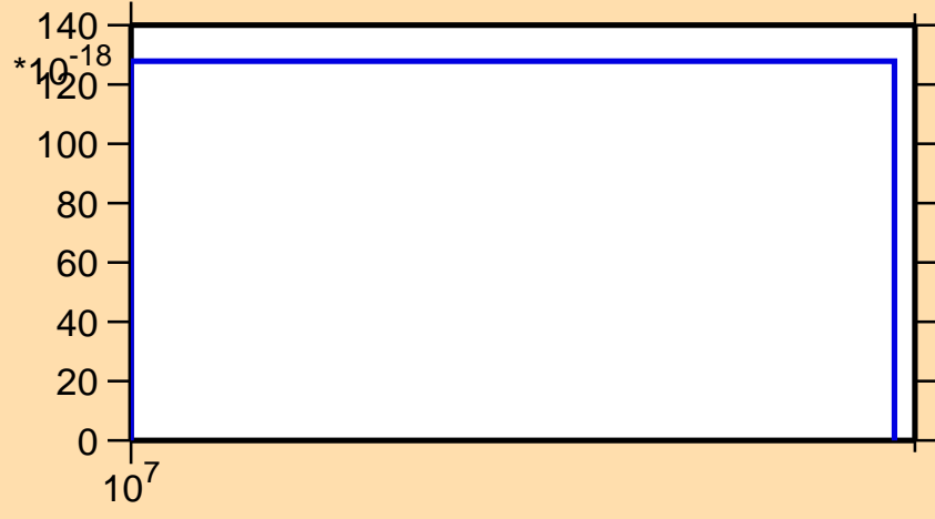
\sigma vs. E for ^{218}\text{Pb} (mt 11)
