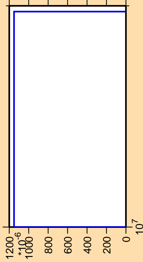
\Delta\sigma/\sigma vs. E for ^{218}\text{Pb} (mt 11)
