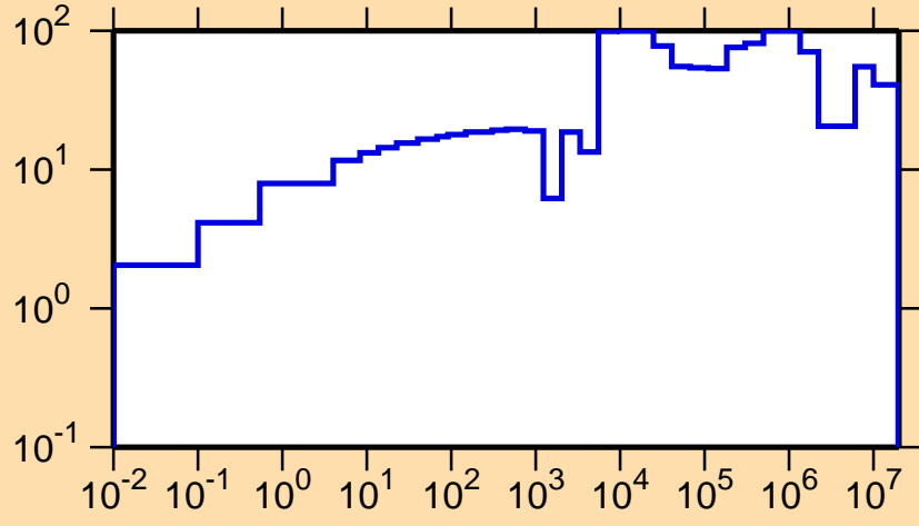
\Delta\sigma/\sigma vs. E for ^{218}\text{Pb}(n,\text{tot.})
