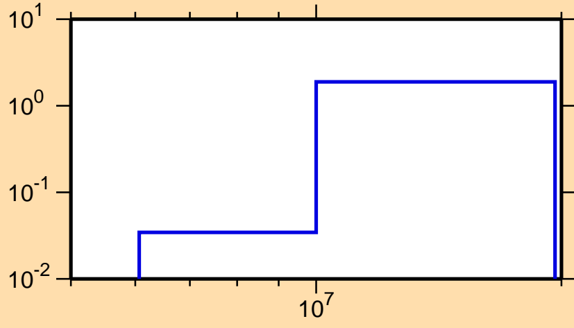
\sigma vs. E for ^{218}\text{Pb}(n,3n)
