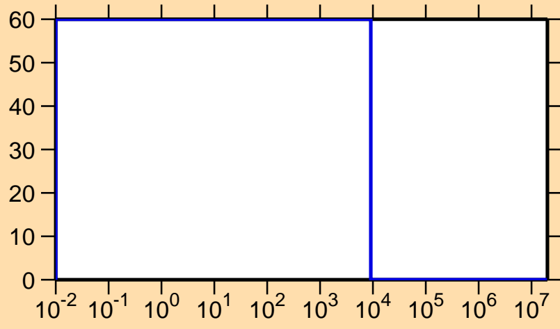
\Delta\sigma/\sigma vs. E for ^{218}\text{Pb}(n,f)
