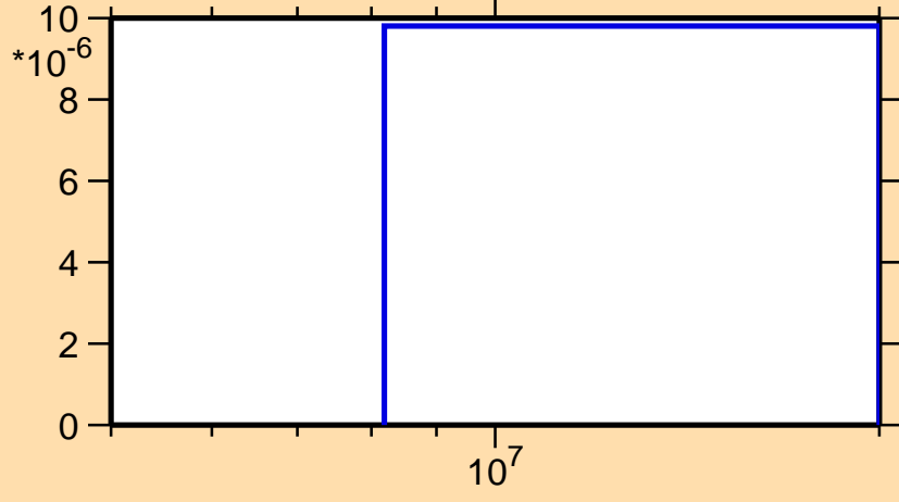
\sigma vs. E for ^{218}\text{Pb}(n,p)
