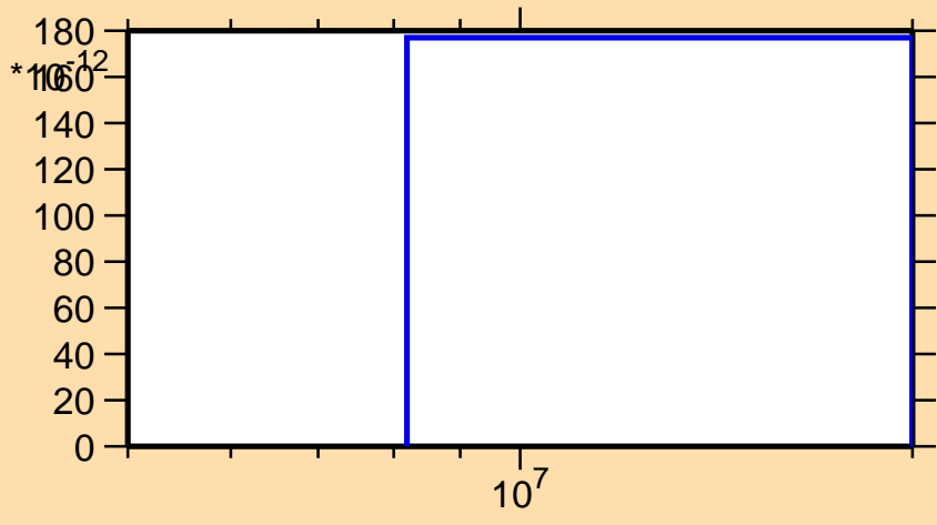
\sigma vs. E for ^{218}\text{Pb}(n,\text{nd})
