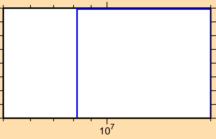
\sigma vs. E for ^{218}\text{Pb}(n,t)
