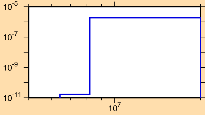
\sigma vs. E for ^{218}\text{Pb}(n,n\alpha)
