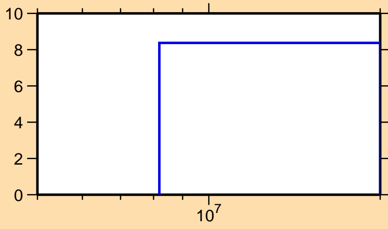
\Delta\sigma/\sigma vs. E for ^{218}\text{Pb}(n,\text{inel.})
