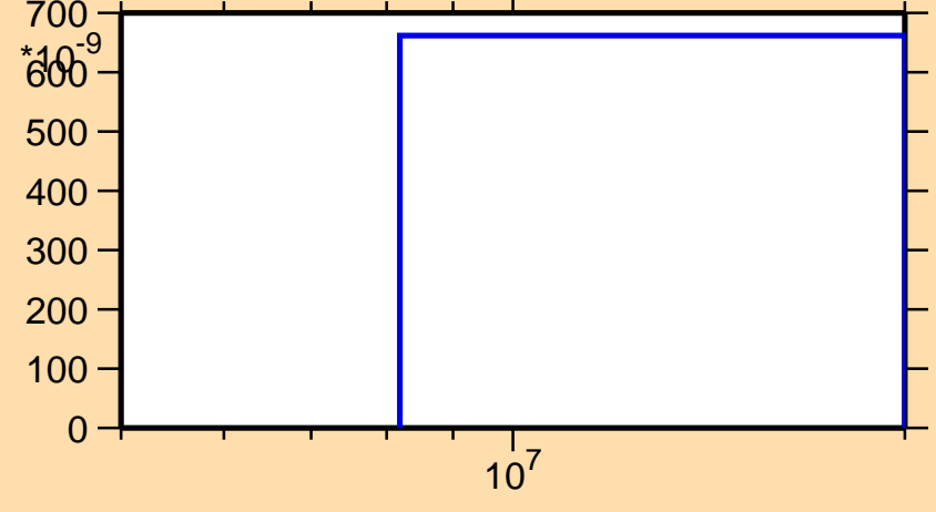
\sigma vs. E for ^{218}\text{Pb}(n,d)
