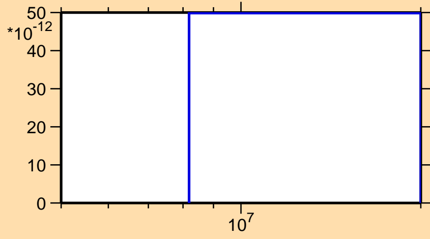
\sigma vs. E for ^{218}\text{Pb}(n,3n\alpha)
