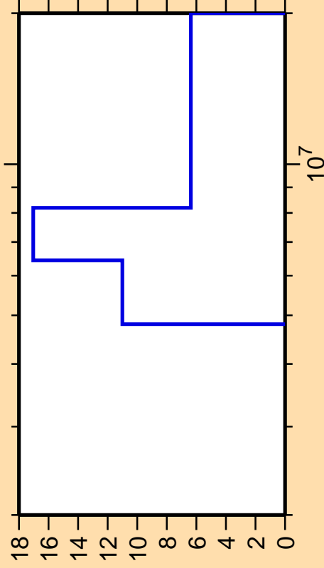
\Delta\sigma/\sigma vs. E for ^{218}\text{Pb}(n,n\text{cont.})
