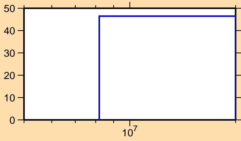
\Delta\sigma/\sigma vs. E for ^{218}\text{Pb}(n,\text{el.})
