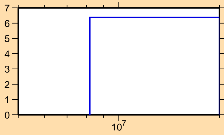
\Delta\sigma/\sigma vs. E for ^{218}\text{Pb}(n,n\text{cont.})
