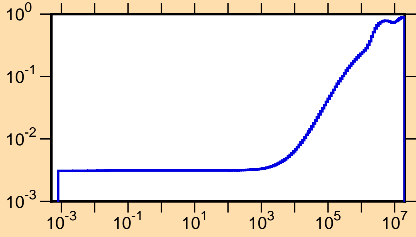
\mu vs. E for ^{219}\text{Pb}(\text{mt251})
