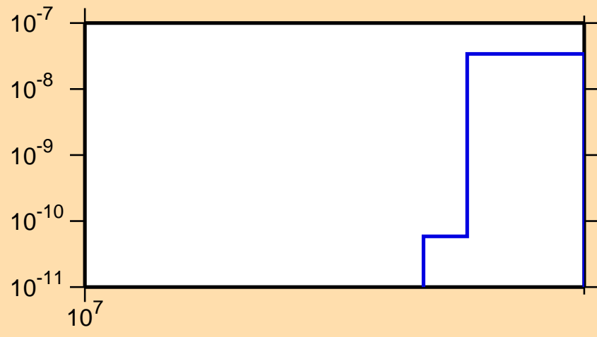
\sigma vs. E for ^{219}\text{Pb}(n,2np)
