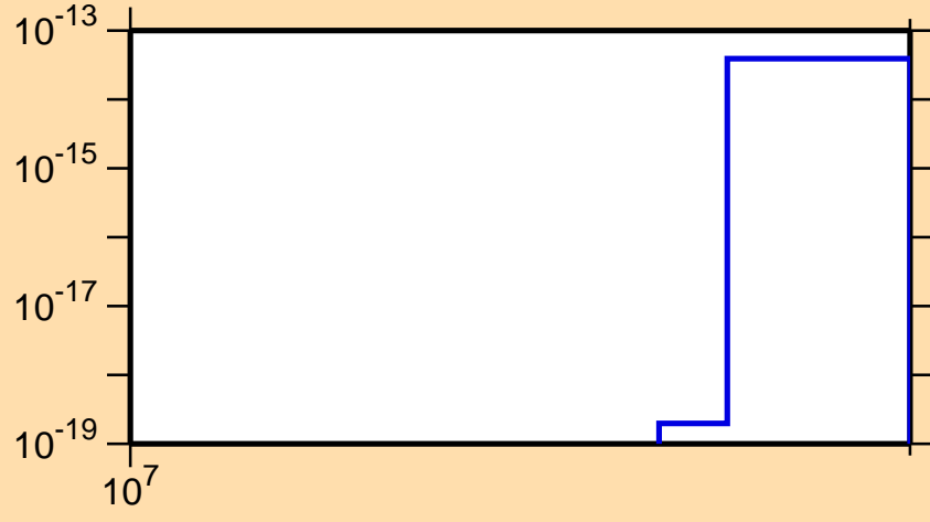
\sigma vs. E for ^{219}\text{Pb} (mt 11)
