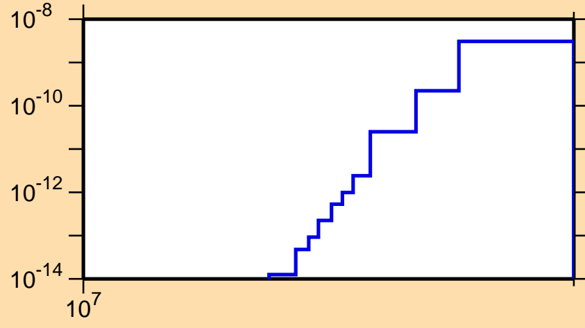
\sigma vs. E for ^{219}\text{Pb}(n,3n\alpha)
