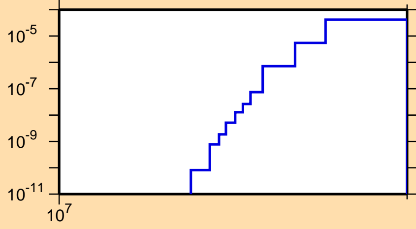
\sigma vs. E for ^{219}\text{Pb}(n,np)
