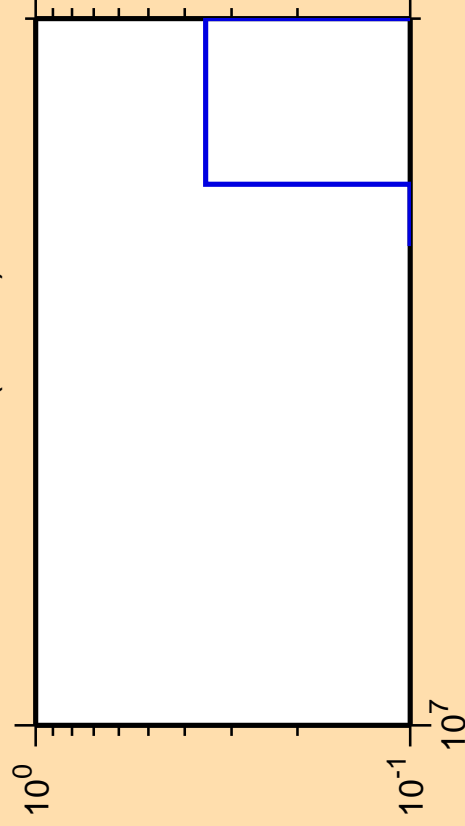
\Delta\sigma/\sigma vs. E for ^{219}\text{Pb} (mt 11)
