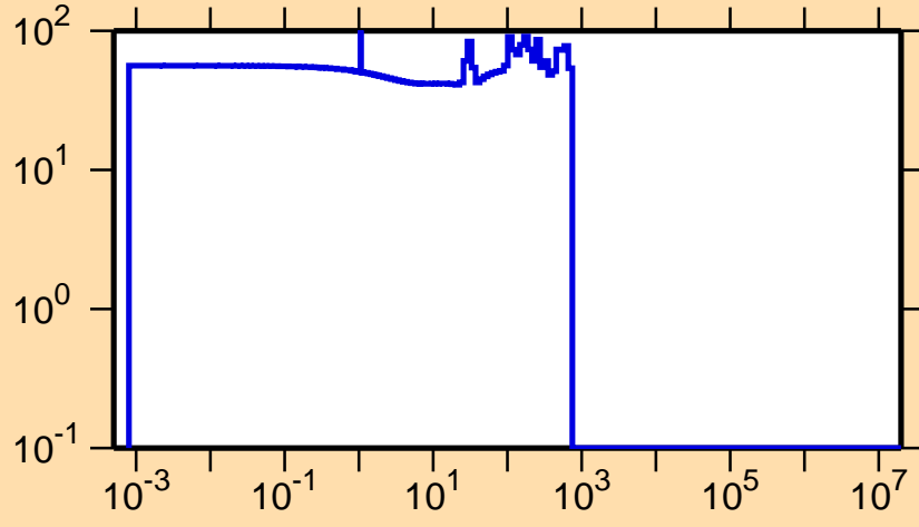
\Delta\sigma/\sigma vs. E for ^{219}\text{Pb}(n,f)
