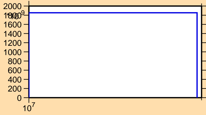
\sigma vs. E for ^{219}\text{Pb}(n,d)
