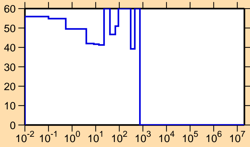
\Delta\sigma/\sigma vs. E for ^{219}\text{Pb}(n,f)
