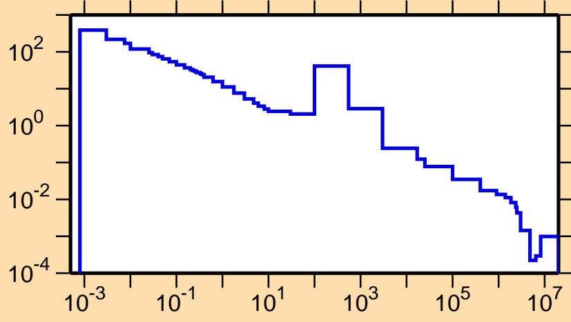
\sigma vs. E for ^{219}\text{Pb}(n,\gamma)
