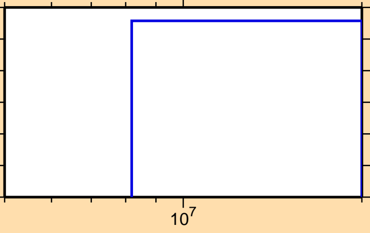
\sigma vs. E for ^{219}\text{Pb}(n,2np)
