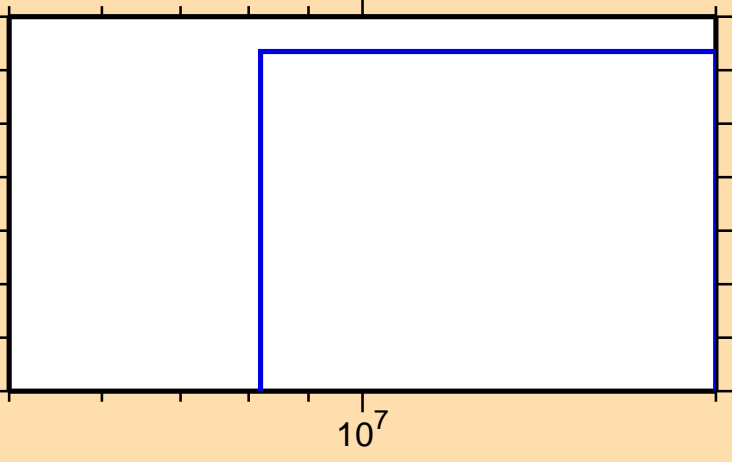
\sigma vs. E for ^{219}\text{Pb}(\text{mt 11})
