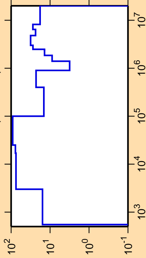
\Delta\sigma/\sigma vs. E for ^{219}\text{Pb}(n,\text{nonel.})
