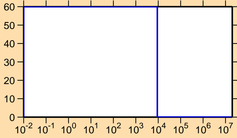
\Delta\sigma/\sigma vs. E for ^{220}\text{Pb}(n,f)
