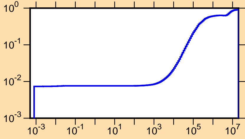
\mu vs. E for ^{92}\text{Pd}(\text{mt251})
