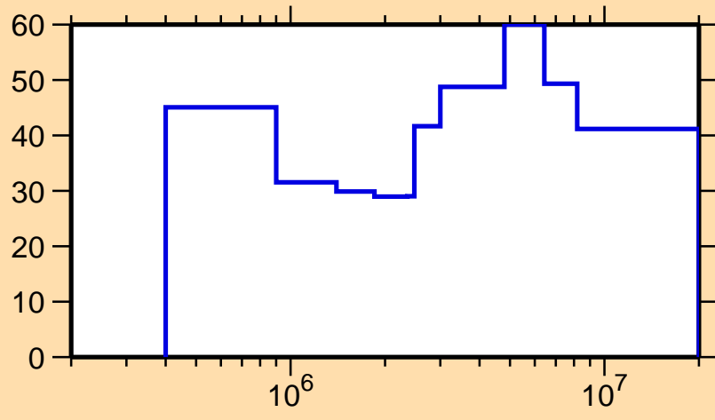
\Delta\sigma/\sigma vs. E for ^{92}\text{Pd}(n,n_1)
