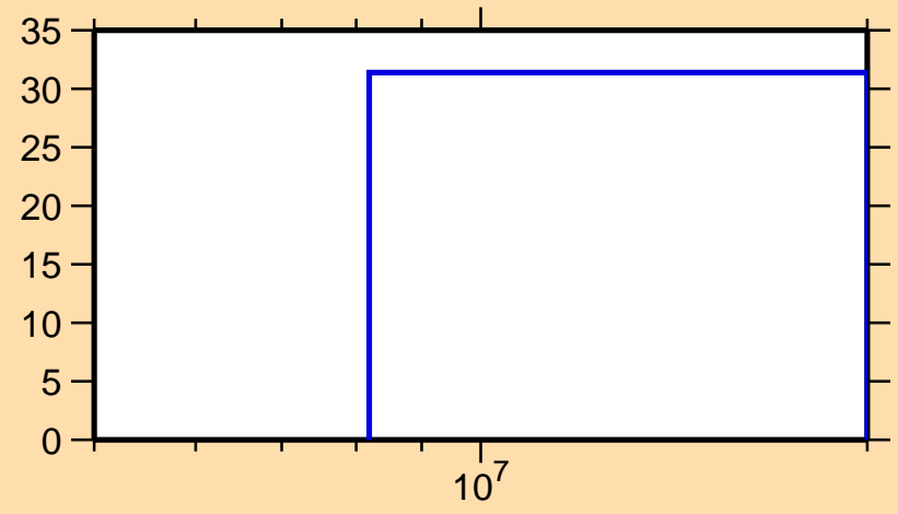
\Delta\sigma/\sigma vs. E for ^{92}\text{Pd}(n,\text{inel.})
