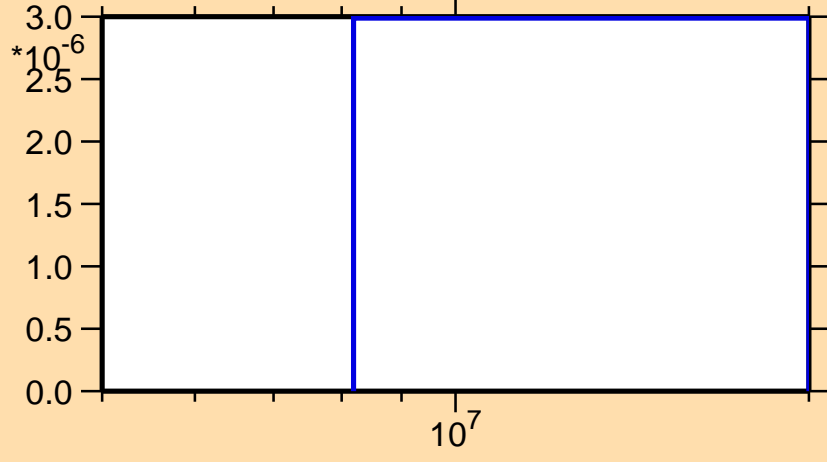
\sigma vs. E for ^{92}\text{Pd}(n,t)
