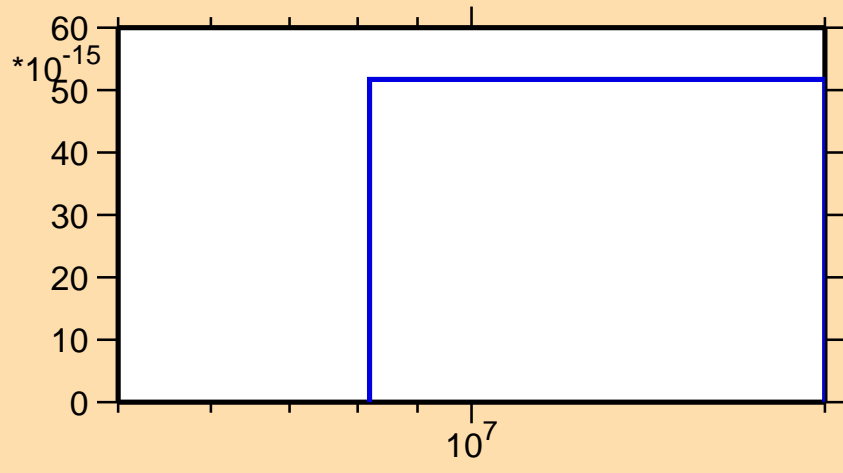
\sigma vs. E for ^{92}\text{Pd}(\text{mt } 34)
