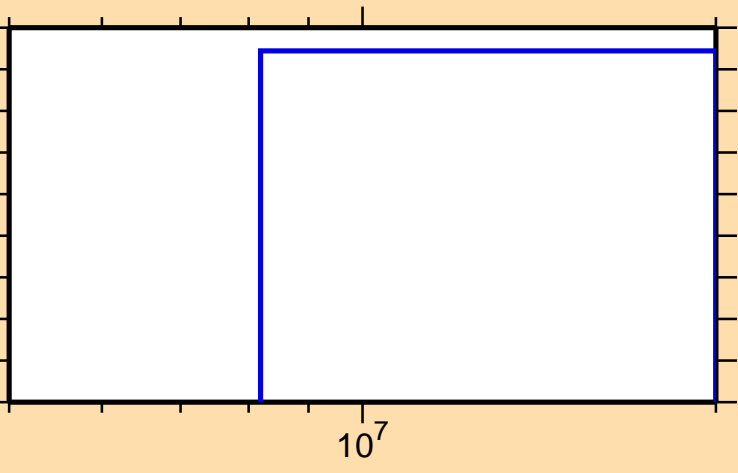
\sigma vs. E for ^{92}\text{Pd}(n,2n)
