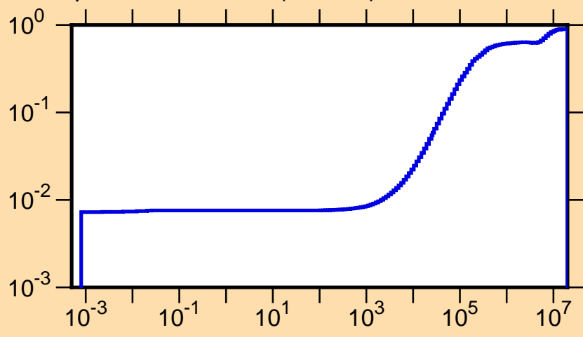
\mu vs. E for ^{93}\text{Pd}(\text{mt251})
