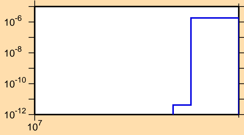
\sigma vs. E for ^{93}\text{Pd}(n,2np)
