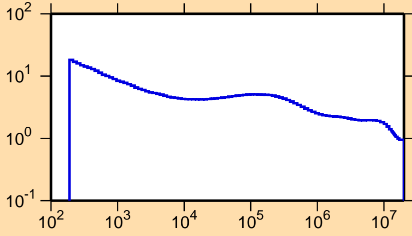
\sigma vs. E for ^{93}\text{Pd}(n,\text{nonel.})
