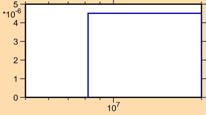
\sigma vs. E for ^{93}\text{Pd}(n,\text{pt})
