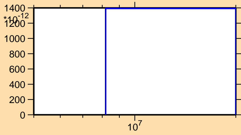
\sigma vs. E for ^{93}\text{Pd}(\text{mt } 45)
