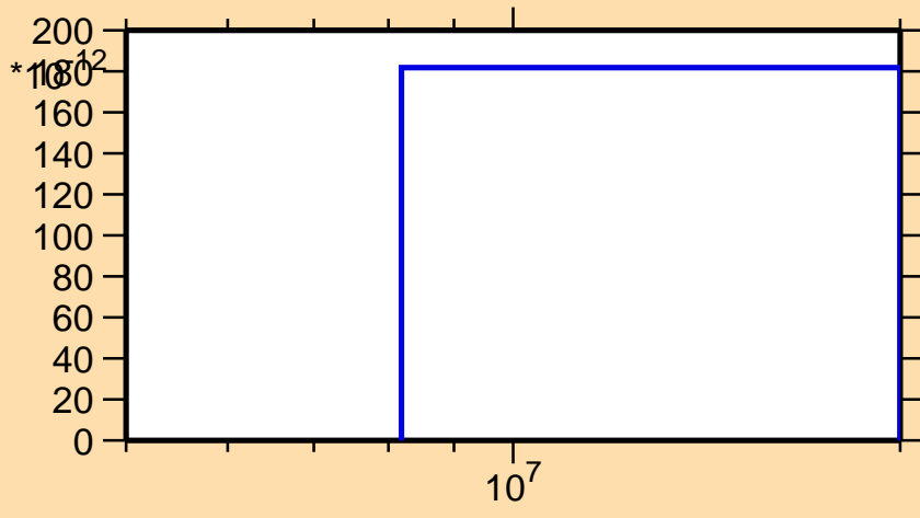
\sigma vs. E for ^{93}\text{Pd}(n,nd)
