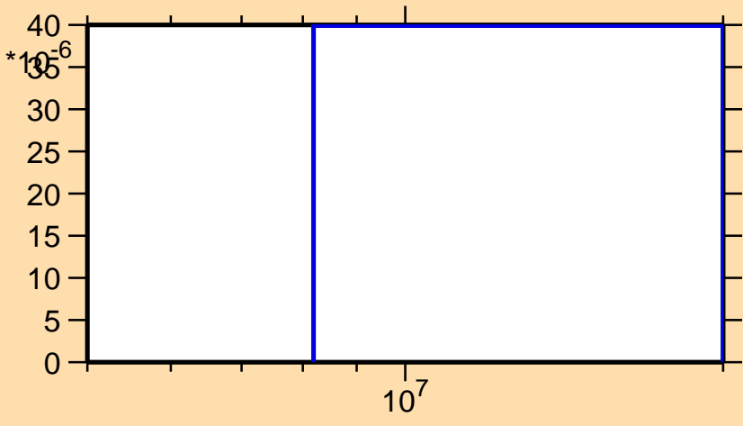
\sigma vs. E for ^{93}\text{Pd}(n,t)
