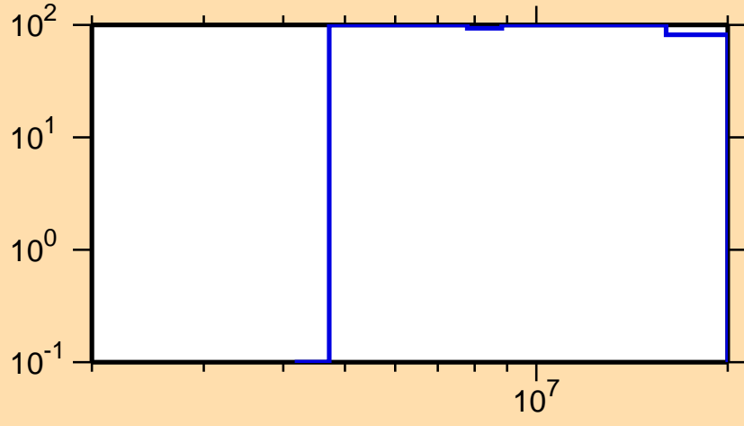
\Delta\sigma/\sigma vs. E for ^{94}\text{Pd}(n,n\text{cont.})
