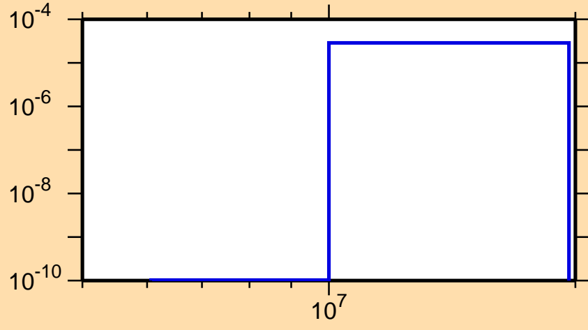
\sigma vs. E for ^{94}\text{Pd}(n,n\alpha)
