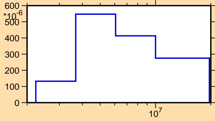
\sigma vs. E for ^{94}\text{Pd}(n,n_3)
