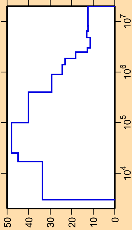
\Delta\sigma/\sigma vs. E for ^{94}\text{Pd}(n,\text{nonel.})
