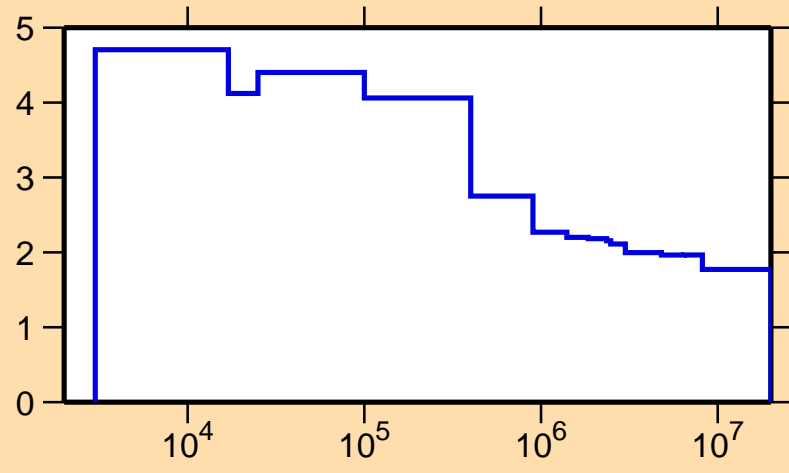
\sigma vs. E for ^{94}\text{Pd}(n,\text{nonel.})
