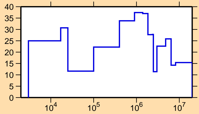
\Delta\sigma/\sigma vs. E for ^{94}\text{Pd}(n,\text{el.})
