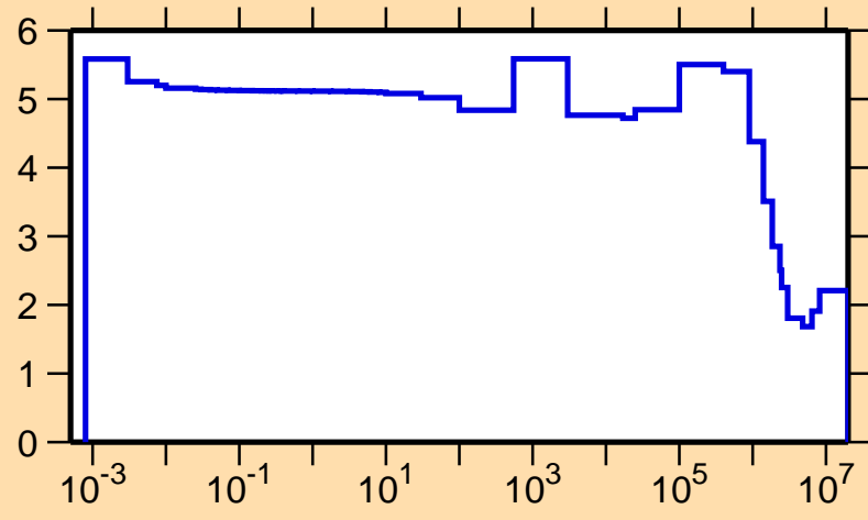
\sigma vs. E for ^{94}\text{Pd}(n,\text{el.})
