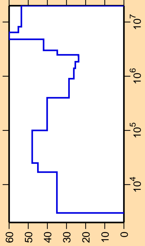
\Delta\sigma/\sigma vs. E for ^{94}\text{Pd}(n,p)
