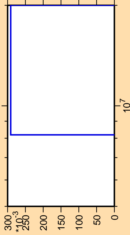
\Delta\sigma/\sigma vs. E for ^{94}\text{Pd}(\text{mt } 34)
