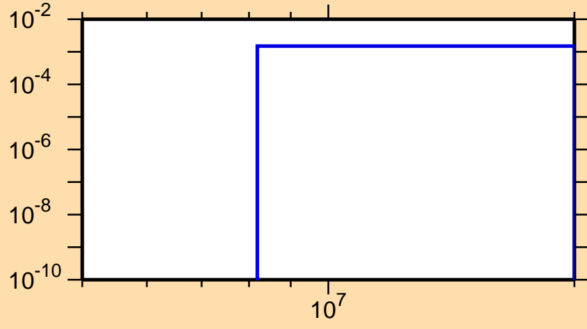
\sigma vs. E for ^{94}\text{Pd}(n,\text{pd})
