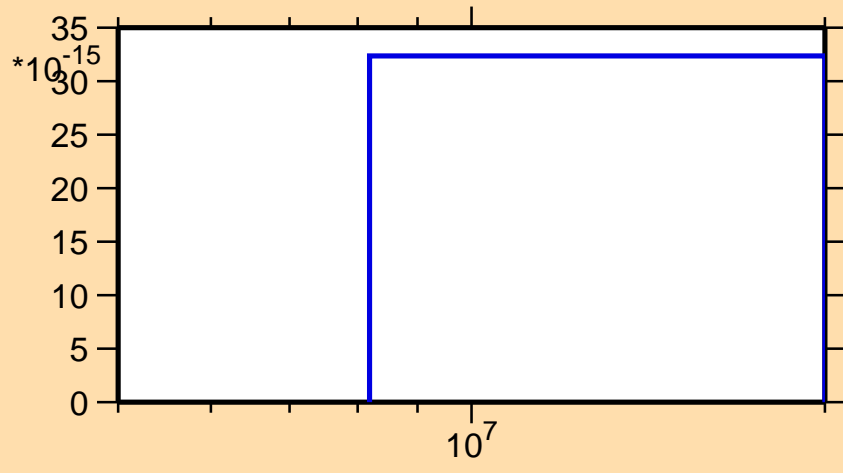
\sigma vs. E for ^{94}\text{Pd}(\text{mt } 34)
