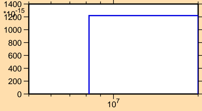
\sigma vs. E for ^{94}\text{Pd}(\text{mt117})
