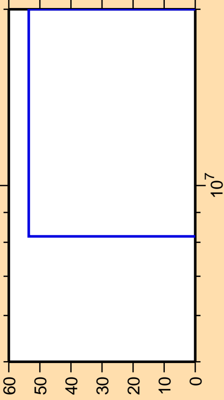
\Delta\sigma/\sigma vs. E for ^{94}\text{Pd}(n,p)
