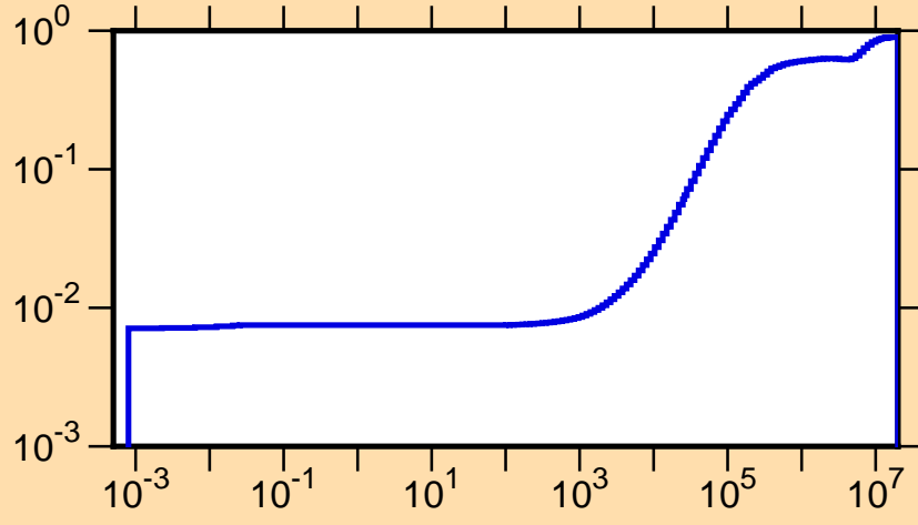
\mu vs. E for ^{95}\text{Pd}(\text{mt251})
