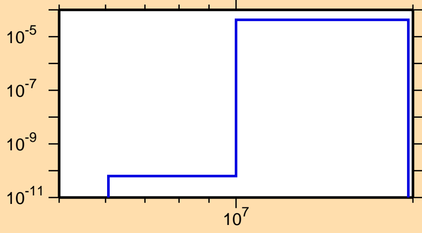
\sigma vs. E for ^{95}\text{Pd}(n,n\alpha)
