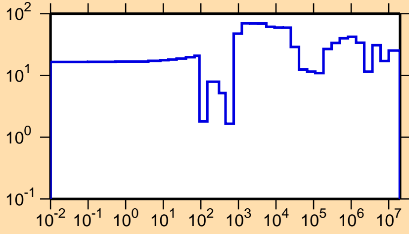
\Delta\sigma/\sigma vs. E for ^{95}\text{Pd}(n,\text{el.})
