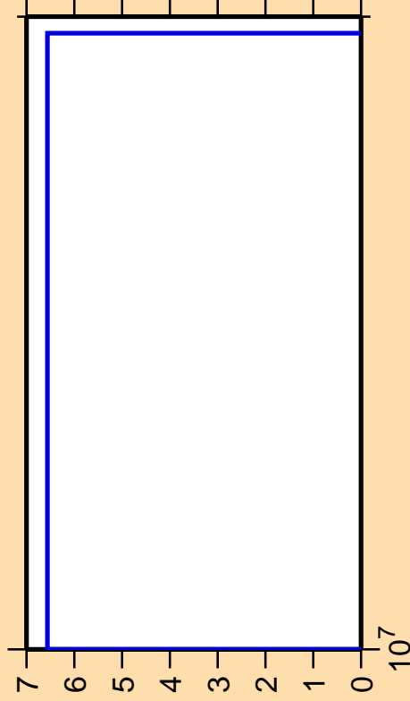
\Delta\sigma/\sigma vs. E for ^{95}\text{Pd}(\text{mt117})
