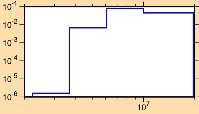
\sigma vs. E for ^{95}\text{Pd}(n,n\text{cont.})
