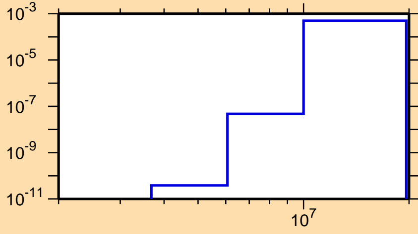
\sigma vs. E for ^{95}\text{Pd}(n,\text{He3})
