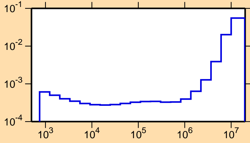
\sigma vs. E for ^{95}\text{Pd}(n,\alpha)
