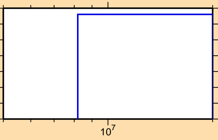
\sigma vs. E for ^{95}\text{Pd}(n,t)
