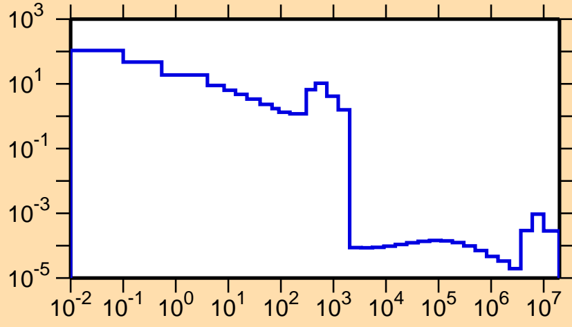
\sigma vs. E for ^{95}\text{Pd}(n,\gamma)
