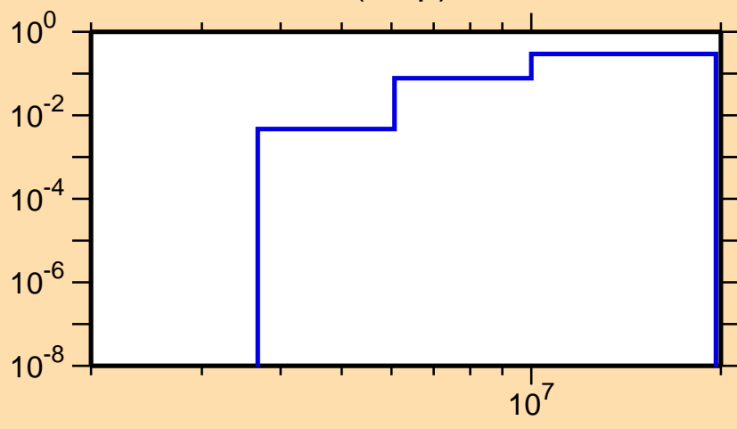
\sigma vs. E for ^{95}\text{Pd}(n,np)
