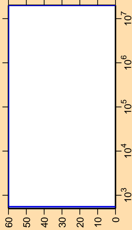
\Delta\sigma/\sigma vs. E for ^{95}\text{Pd}(n,n_2)
