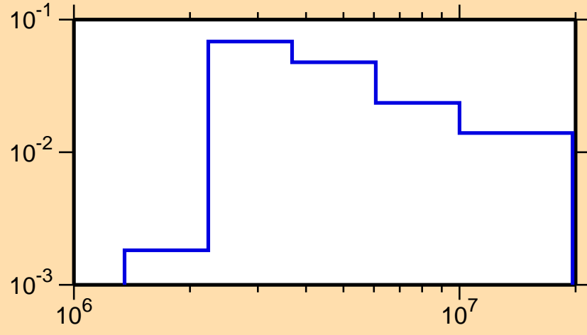
\sigma vs. E for ^{96}\text{Pd}(n,n_2)
