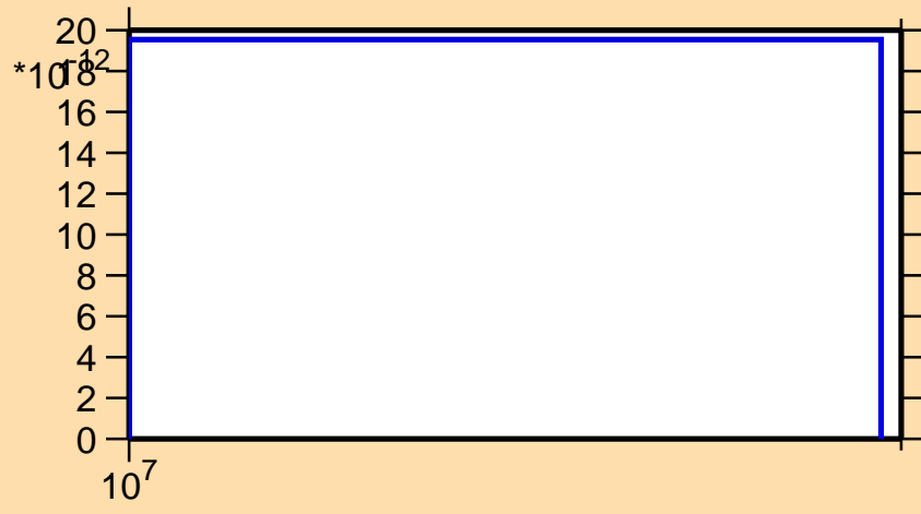
\sigma vs. E for ^{96}\text{Pd}(\text{mt } 45)
