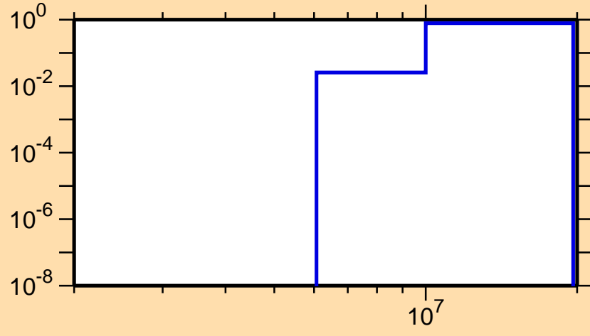
\sigma vs. E for ^{96}\text{Pd}(n,np)
