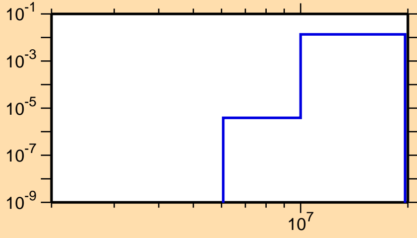
\sigma vs. E for ^{96}\text{Pd}(n,p\alpha)
