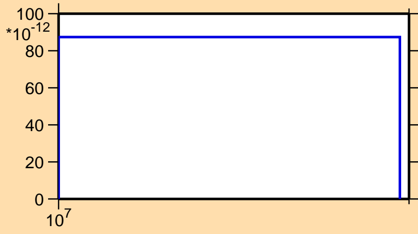
\sigma vs. E for ^{96}\text{Pd}(n,\text{pt})
