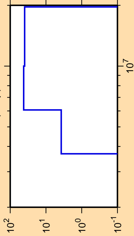
\Delta\sigma/\sigma vs. E for ^{96}\text{Pd}(n,np)
