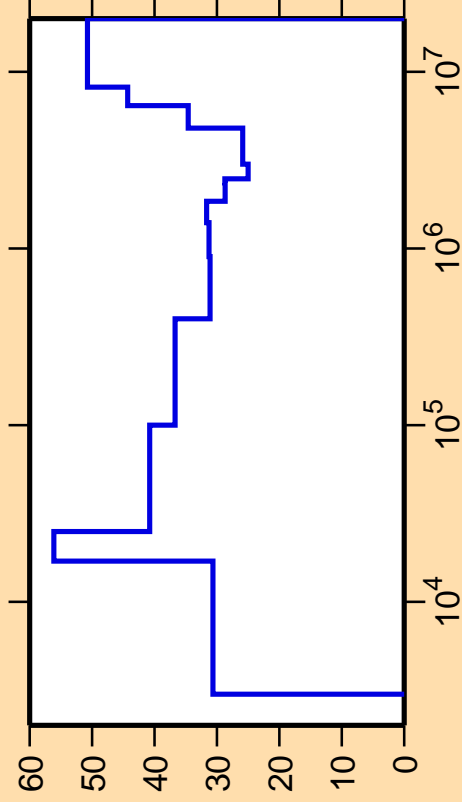
\Delta\sigma/\sigma vs. E for ^{96}\text{Pd}(n,p)
