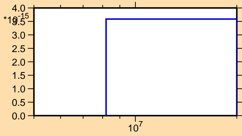
\sigma vs. E for ^{96}\text{Pd}(n,2np)
