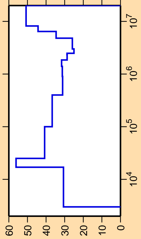
\Delta\sigma/\sigma vs. E for ^{96}\text{Pd}(n,p)
