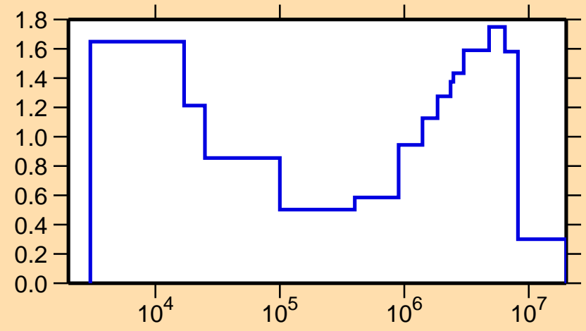
\sigma vs. E for ^{96}\text{Pd}(n,p)
