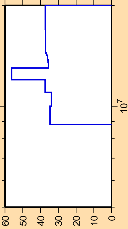
\Delta\sigma/\sigma vs. E for ^{97}\text{Pd}(n,n_1)
