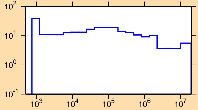
\Delta\sigma/\sigma vs. E for ^{97}\text{Pd}(n,\text{el.})
