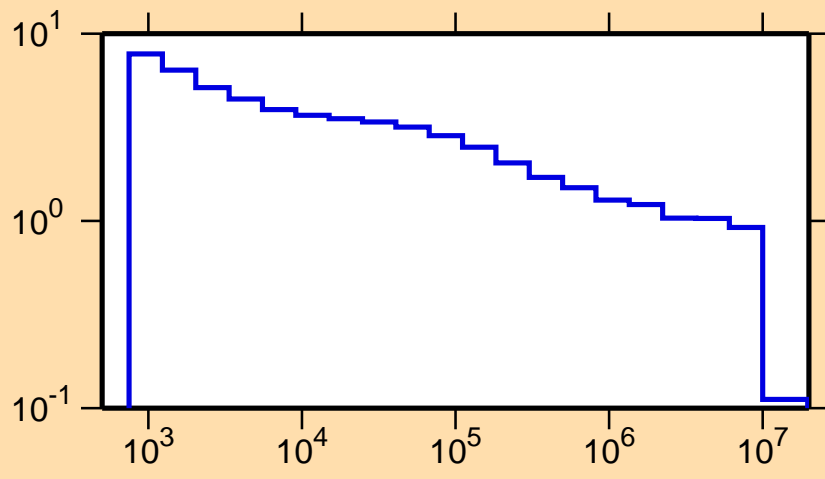
\sigma vs. E for ^{97}\text{Pd}(n,p)
