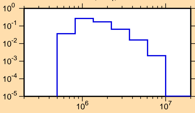
\sigma vs. E for ^{97}\text{Pd}(n,n_1)
