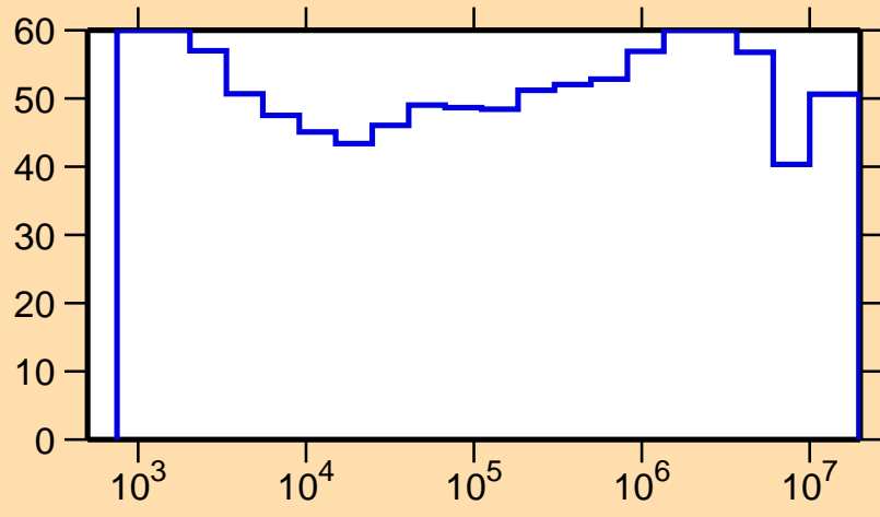
\Delta\sigma/\sigma vs. E for ^{97}\text{Pd}(n,\gamma)
