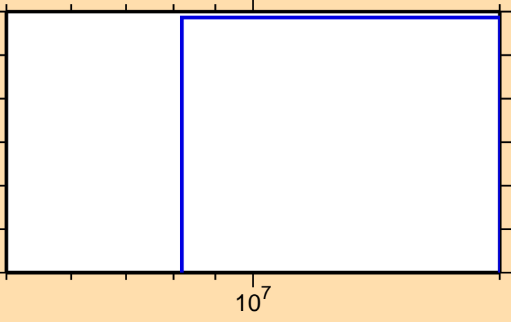
\sigma vs. E for ^{97}\text{Pd}(n,2n)
