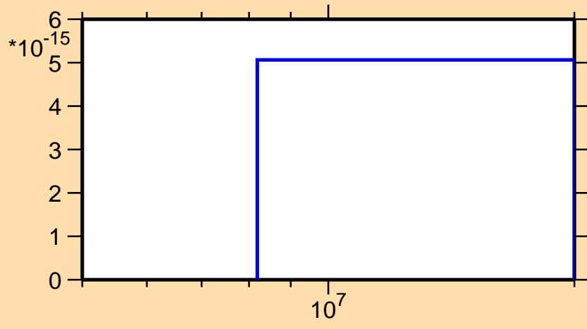
\sigma vs. E for ^{97}\text{Pd}(n,2n\alpha)
