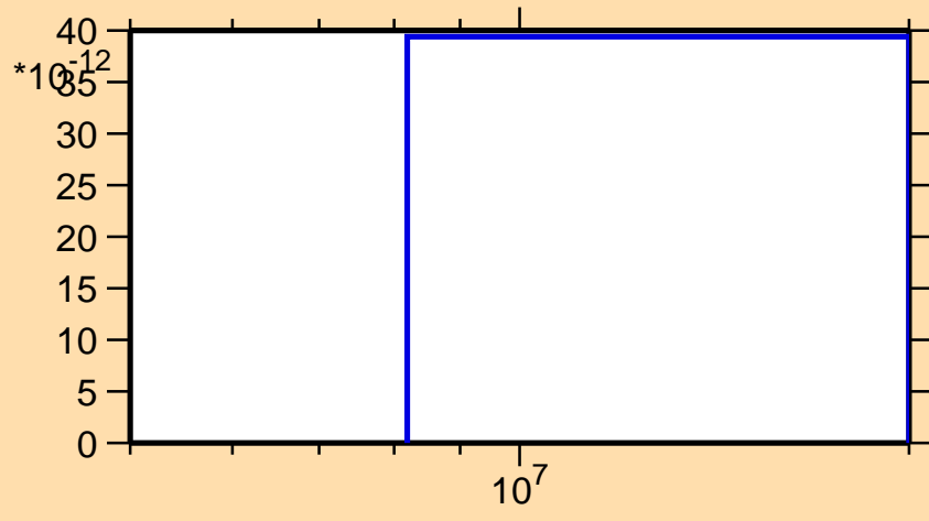
\sigma vs. E for ^{97}\text{Pd}(\text{mt117})
