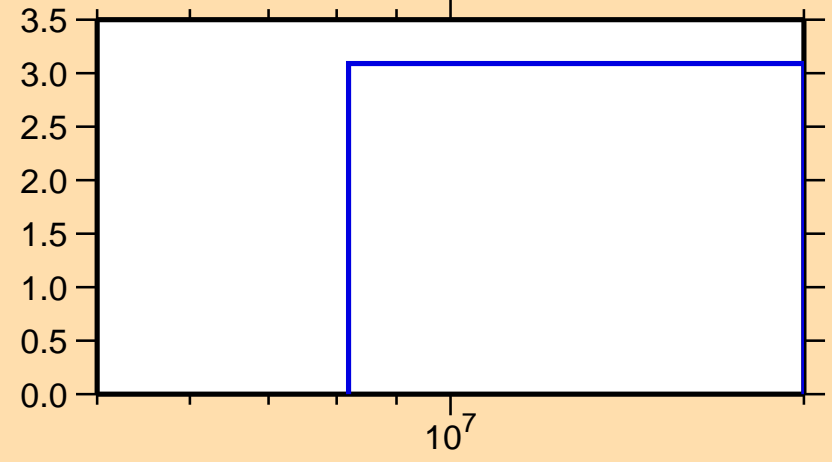
\Delta\sigma/\sigma vs. E for ^{97}\text{Pd}(n,\text{tot.})
