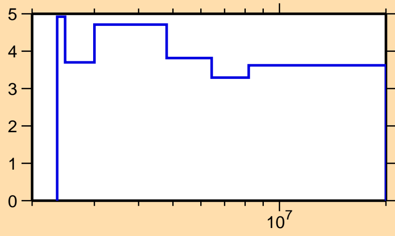
\Delta\sigma/\sigma vs. E for ^{97}\text{Pd}(n,n\text{onel.})
