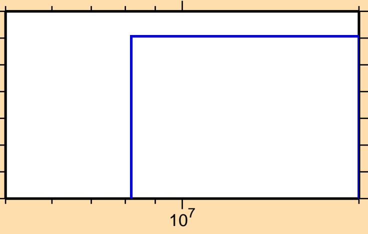
\sigma vs. E for ^{97}\text{Pd}(n,\text{pt})
