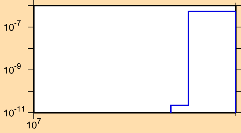
\sigma vs. E for ^{98}\text{Pd}(n,\text{nd})
