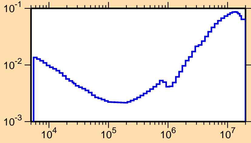
\sigma vs. E for ^{98}\text{Pd}(n,\alpha)
