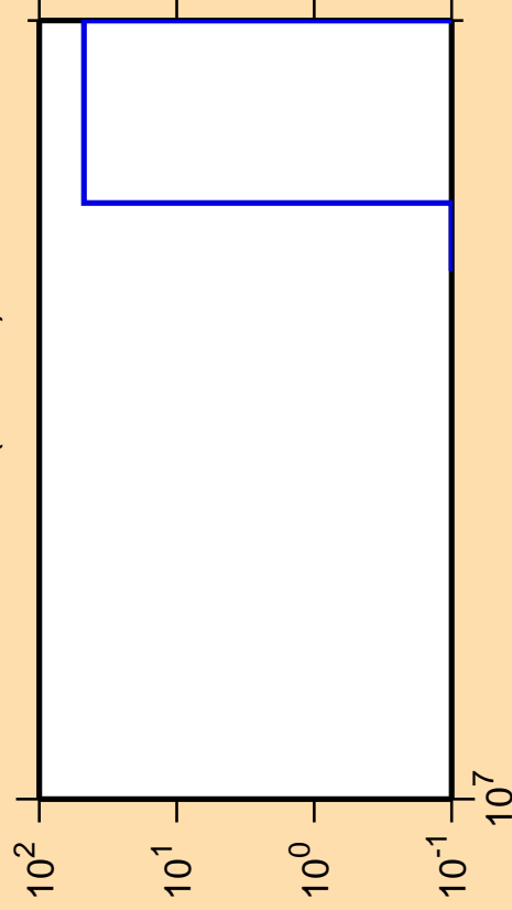
\Delta\sigma/\sigma vs. E for ^{98}\text{Pd}(n,2n\alpha)
