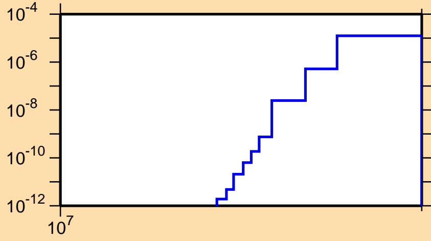
\sigma vs. E for ^{98}\text{Pd}(\text{mt } 45)
