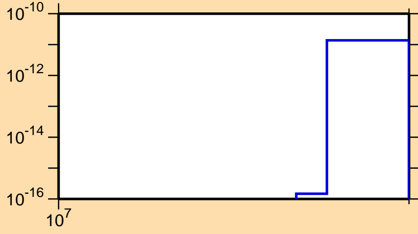
\sigma vs. E for ^{98}\text{Pd}(n,2n\alpha)
