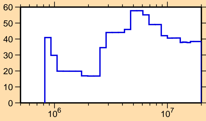
\Delta\sigma/\sigma vs. E for ^{98}\text{Pd}(n,n_1)
