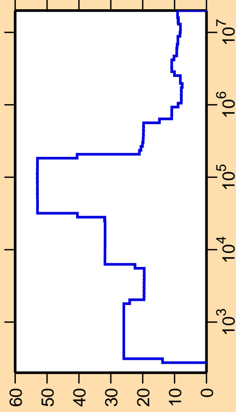
\Delta\sigma/\sigma vs. E for ^{99}\text{Pd}(n,\text{nonel.})
