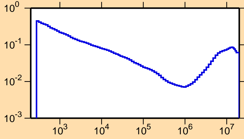
\sigma vs. E for ^{99}\text{Pd}(n,\alpha)
