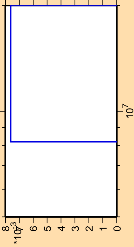
\Delta\sigma/\sigma vs. E for ^{99}\text{Pd}(n,nt)
