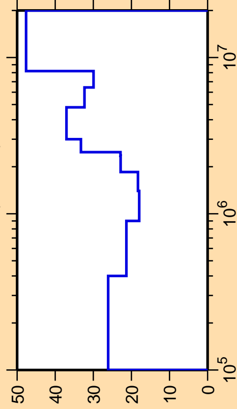
\Delta\sigma/\sigma vs. E for ^{99}\text{Pd}(n,\text{inel.})
