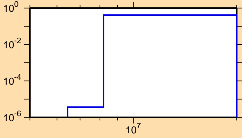
\sigma vs. E for ^{99}\text{Pd}(n,np)
