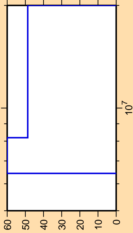
\Delta\sigma/\sigma vs. E for ^{99}\text{Pd}(n,np)
