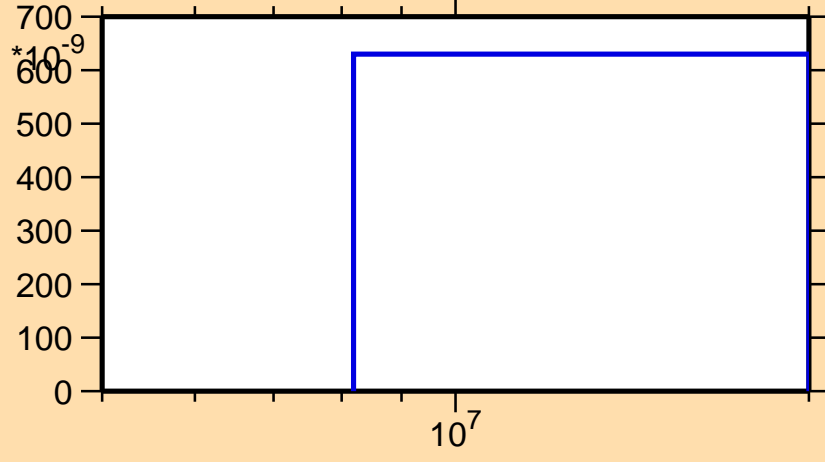
\sigma vs. E for ^{99}\text{Pd}(n,2n\alpha)
