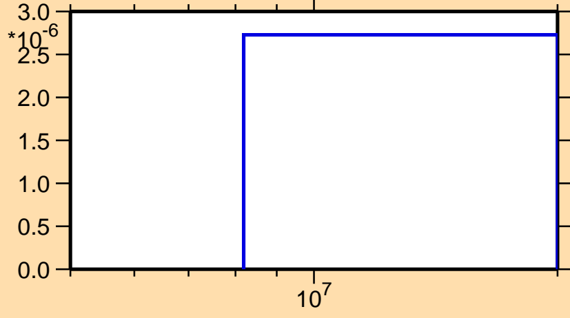
\sigma vs. E for ^{99}\text{Pd}(n,\text{pd})
