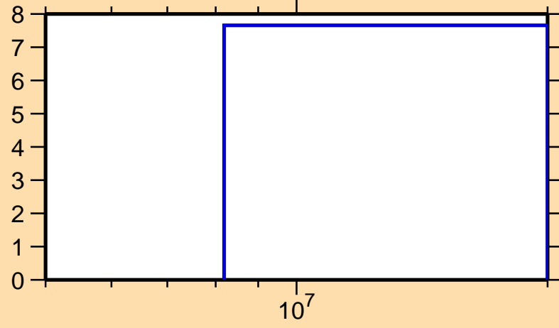
\Delta\sigma/\sigma vs. E for ^{99}\text{Pd}(n,\text{el.})
