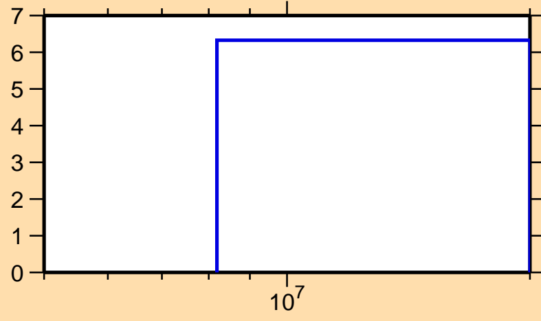
\Delta\sigma/\sigma vs. E for ^{99}\text{Pd}(n,\text{tot.})
