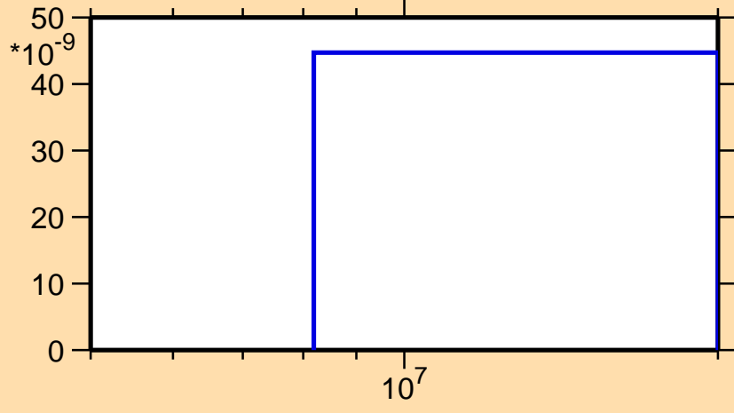
\sigma vs. E for ^{99}\text{Pd}(\text{mt } 45)
