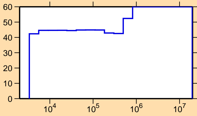
\Delta\sigma/\sigma vs. E for ^{100}\text{Pd}(n,\gamma)
