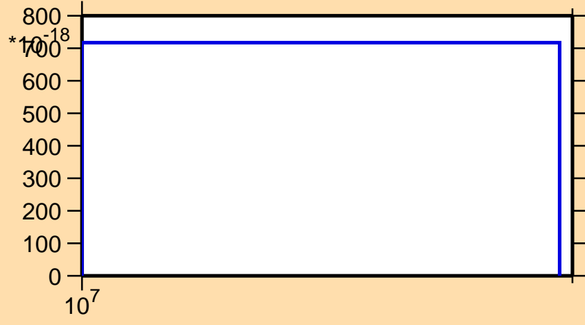
\sigma vs. E for ^{100}\text{Pd}(n,nt)
