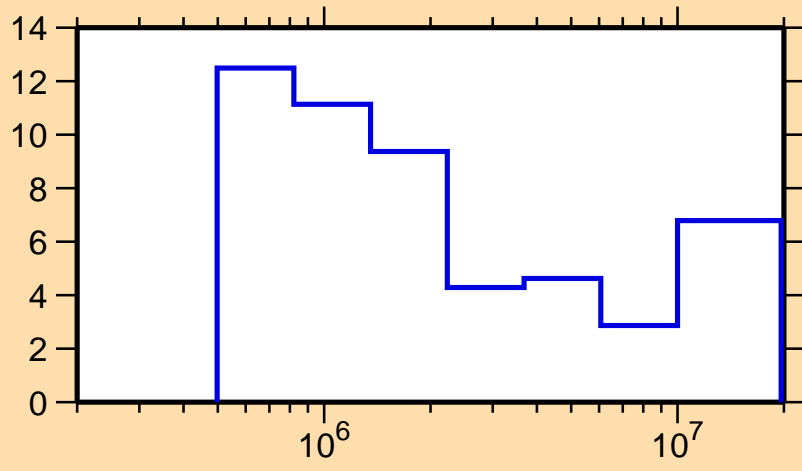
\Delta\sigma/\sigma vs. E for ^{100}\text{Pd}(n,\text{tot.})
