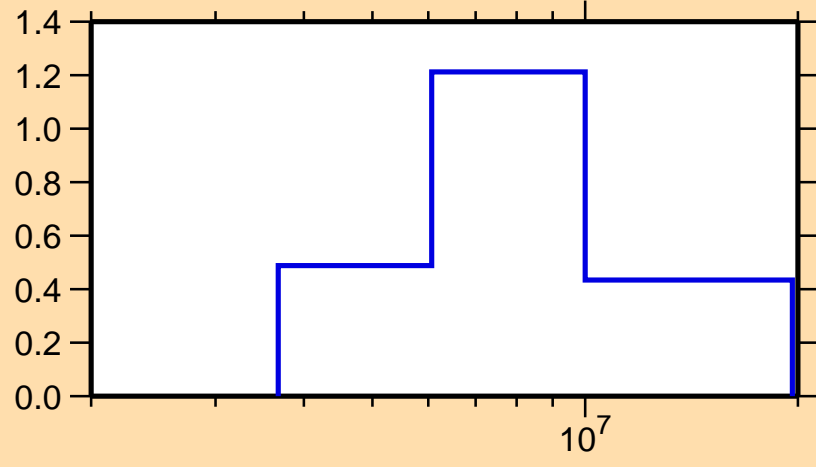
\sigma vs. E for ^{100}\text{Pd}(n,n\text{cont.})
