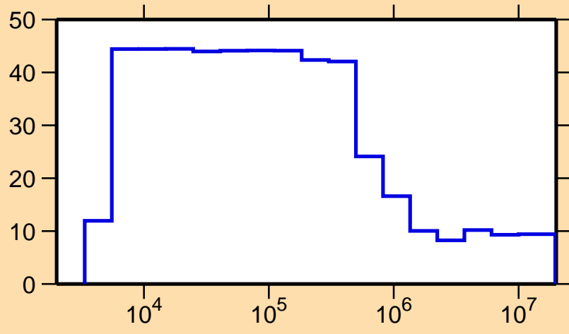
\Delta\sigma/\sigma vs. E for ^{100}\text{Pd}(n,\text{nonel.})
