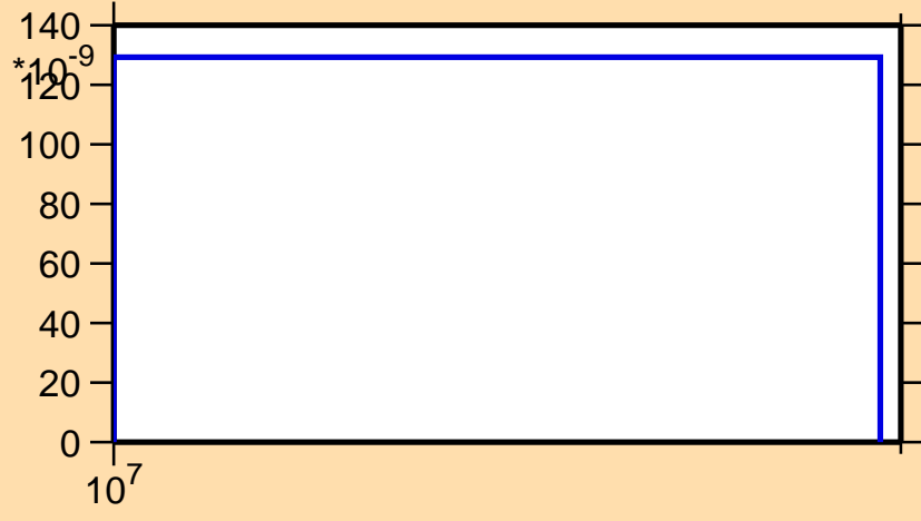
\sigma vs. E for ^{100}\text{Pd}(n,\text{pd})
