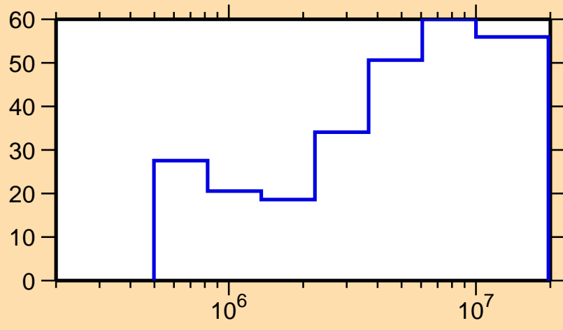
\Delta\sigma/\sigma vs. E for ^{100}\text{Pd}(n,n_1)
