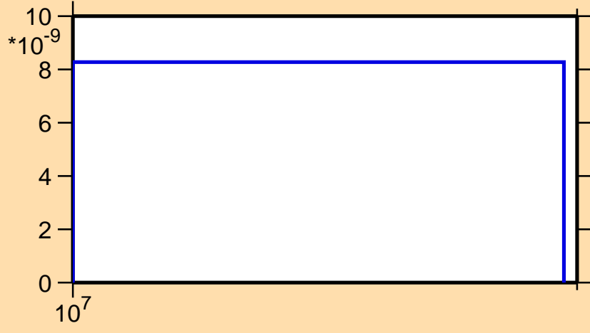
\sigma vs. E for ^{100}\text{Pd}(n,2n\alpha)
