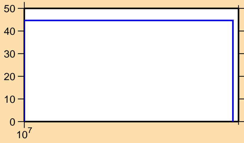
\Delta\sigma/\sigma vs. E for ^{100}\text{Pd}(n,2n)
