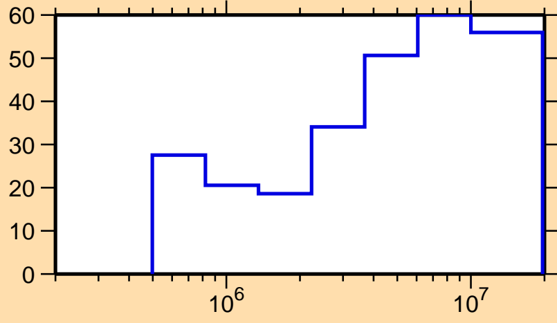
\Delta\sigma/\sigma vs. E for ^{100}\text{Pd}(n,n_1)
