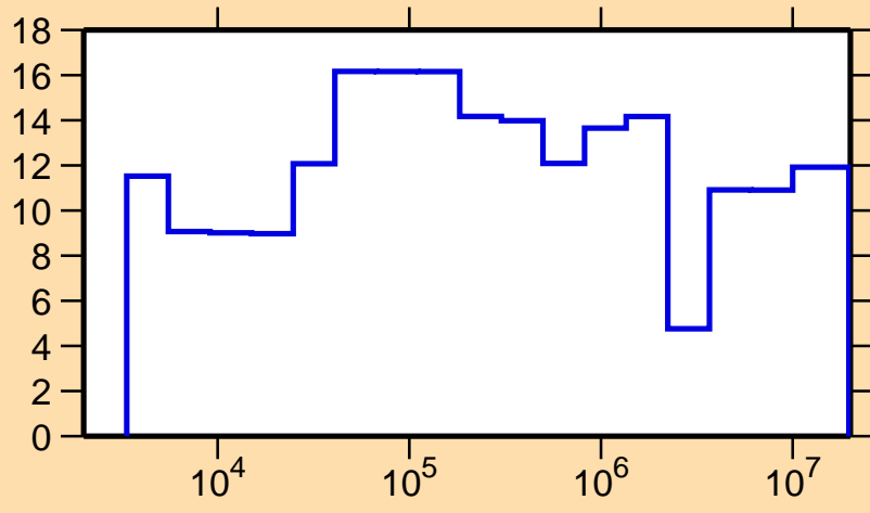
\Delta\sigma/\sigma vs. E for ^{100}\text{Pd}(n,\text{el.})
