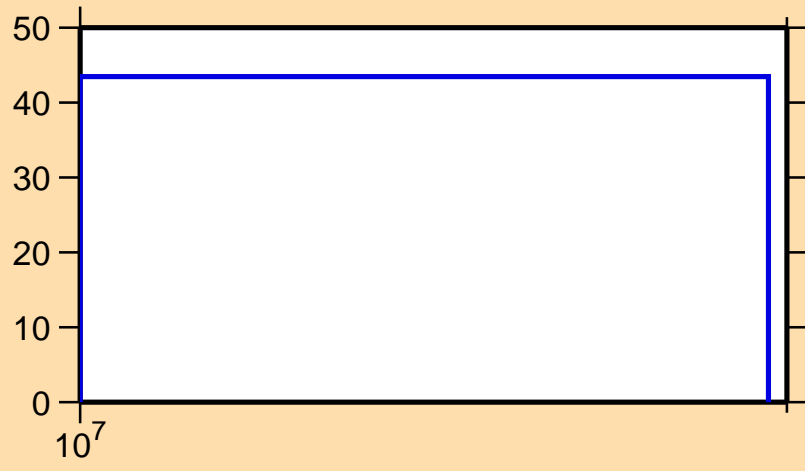
\Delta\sigma/\sigma vs. E for ^{100}\text{Pd}(n,\text{inel.})
