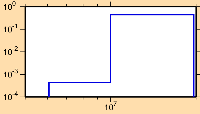
\sigma vs. E for ^{100}\text{Pd}(n,np)
