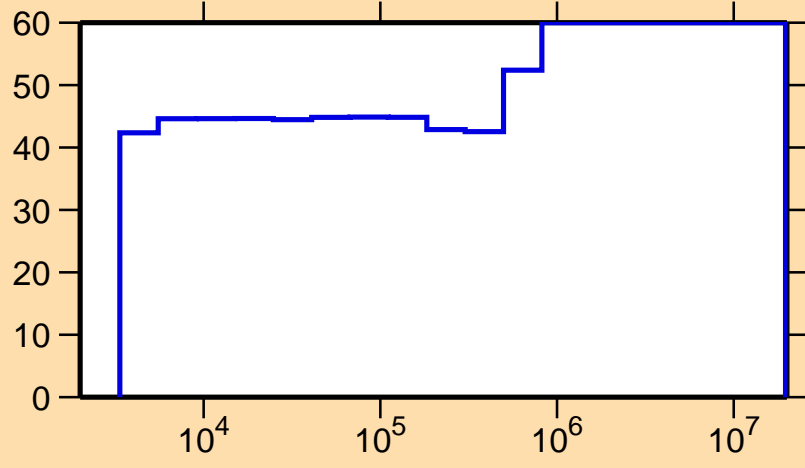
\Delta\sigma/\sigma vs. E for ^{100}\text{Pd}(n,\gamma)
