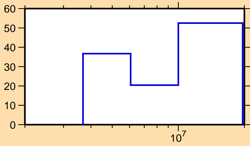
\Delta\sigma/\sigma vs. E for ^{100}\text{Pd}(n,n\text{cont.})
