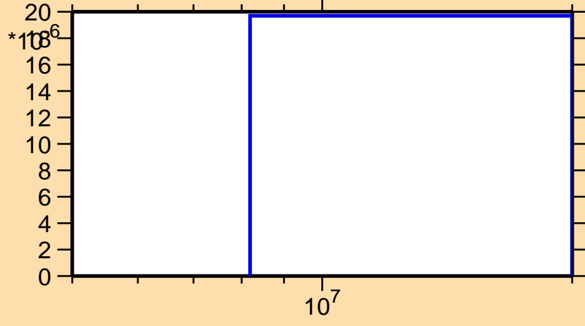
\sigma vs. E for ^{100}\text{Pd}(n,t)
