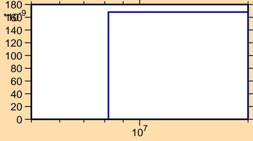
\sigma vs. E for ^{100}\text{Pd}(n,\text{He}3)
