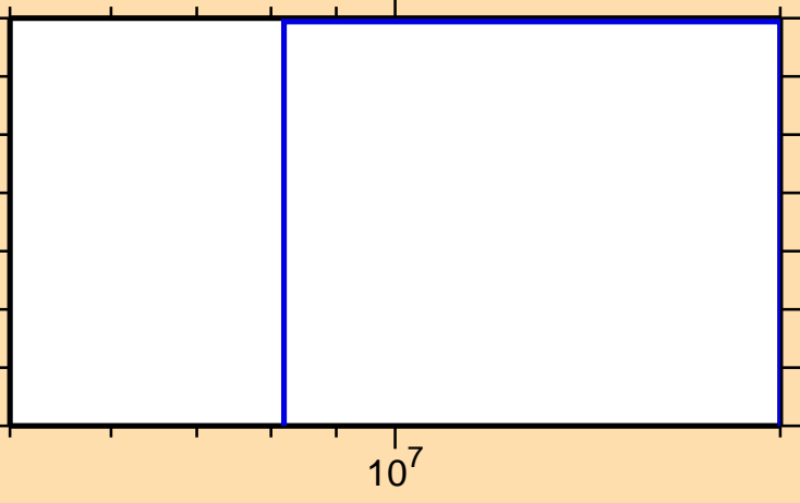
\sigma vs. E for ^{101}\text{Pd}(n,nt)
