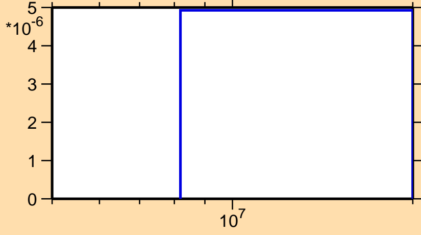
\sigma vs. E for ^{101}\text{Pd}(n,2np)
