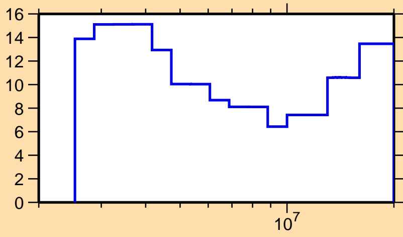
\Delta\sigma/\sigma vs. E for ^{102}\text{Pd}(n, el.)
