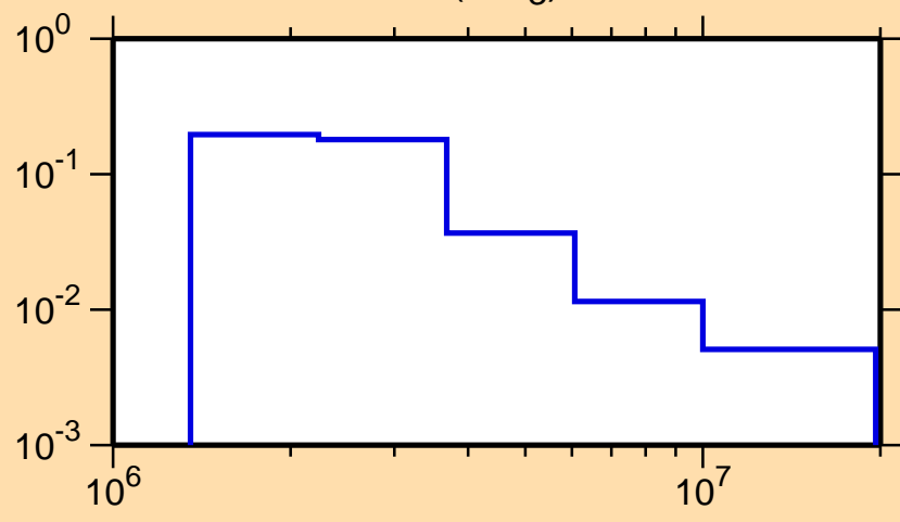
\sigma vs. E for ^{102}\text{Pd}(n,n_3)
