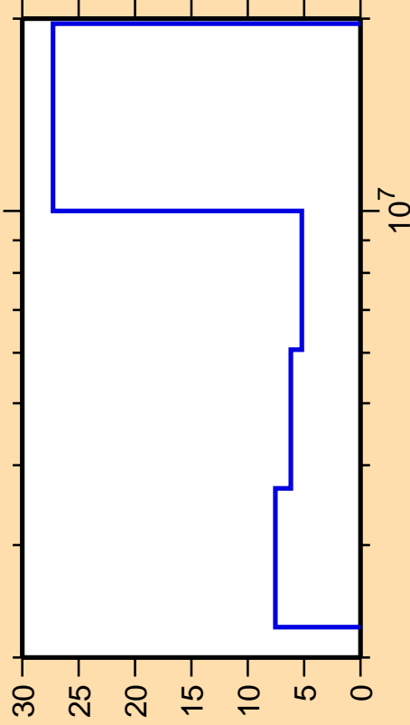
\Delta\sigma/\sigma vs. E for ^{102}\text{Pd}(n,n\text{cont.})
