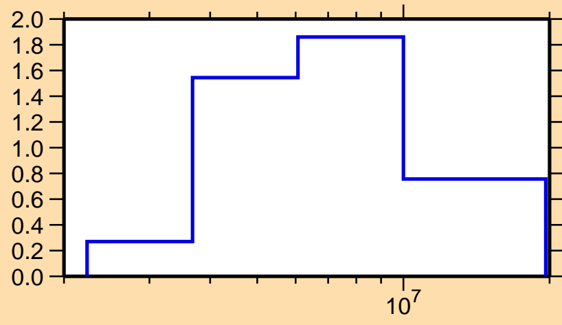
\sigma vs. E for ^{102}\text{Pd}(n,n\text{cont.})
