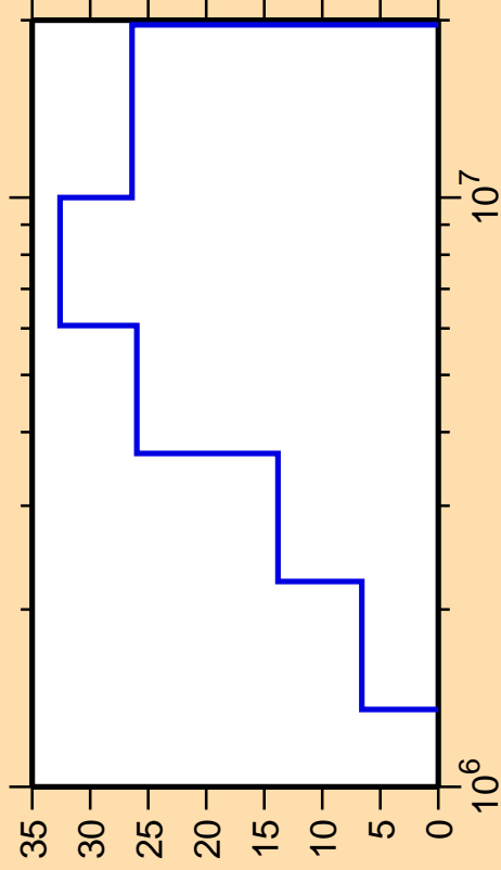
\Delta\sigma/\sigma vs. E for ^{102}\text{Pd}(n,n_3)
