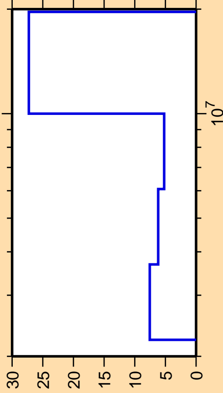
\Delta\sigma/\sigma vs. E for ^{102}\text{Pd}(n,\text{ncont.})
