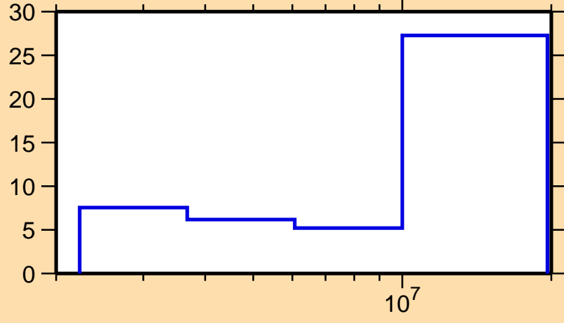
\Delta\sigma/\sigma vs. E for ^{102}\text{Pd}(n,n\text{cont.})
