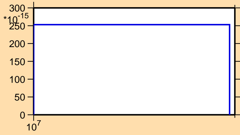
\sigma vs. E for ^{102}\text{Pd}(\text{mt } 45)
