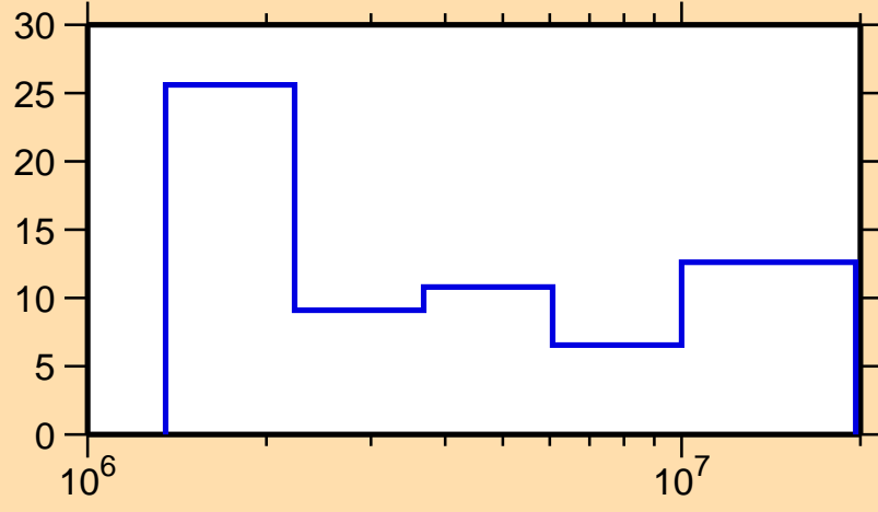
\Delta\sigma/\sigma vs. E for ^{103}\text{Pd}(n, el.)
