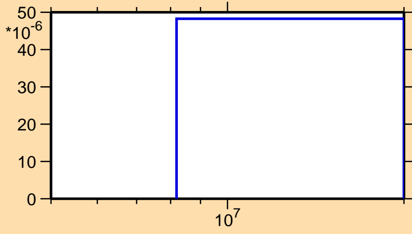
\sigma vs. E for ^{103}\text{Pd}(n,t)
