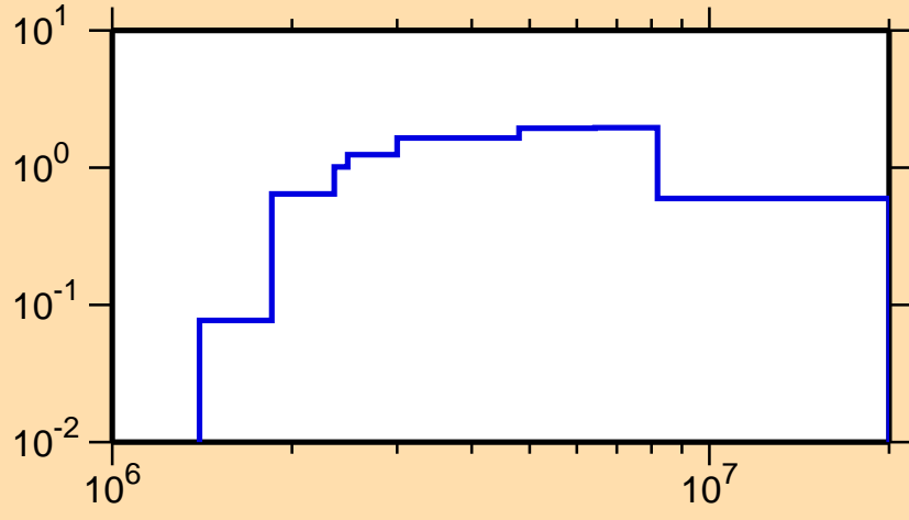
\sigma vs. E for ^{103}\text{Pd}(n,n\text{cont.})
