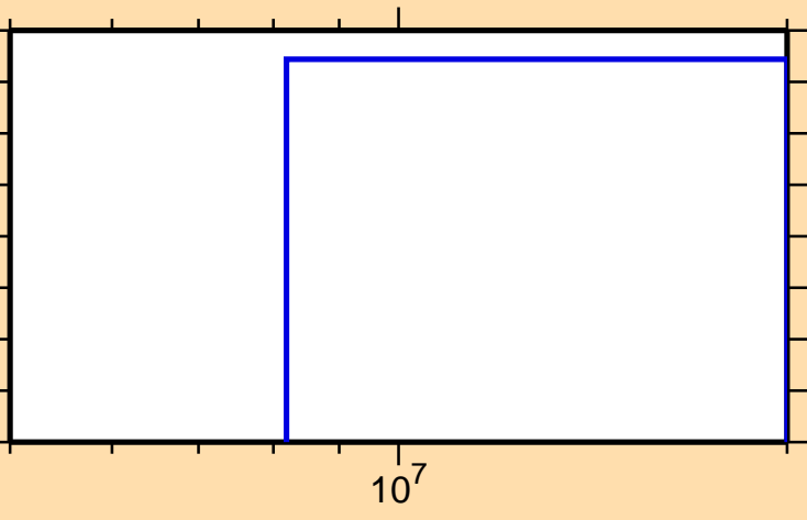
\sigma vs. E for ^{103}\text{Pd}(n,3n)
