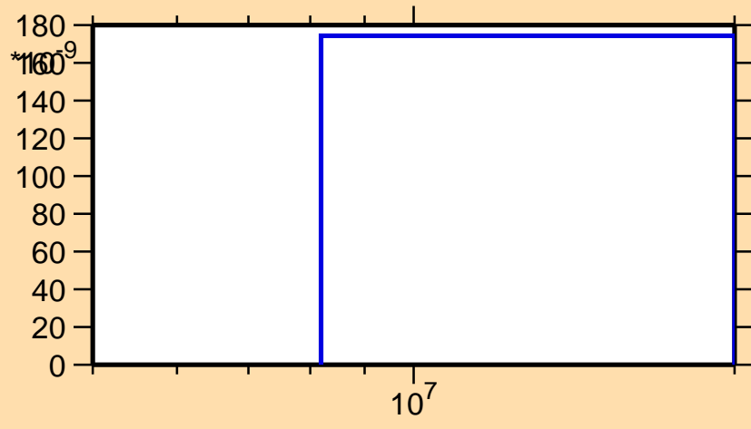
\sigma vs. E for ^{103}\text{Pd}(n,p\alpha)
