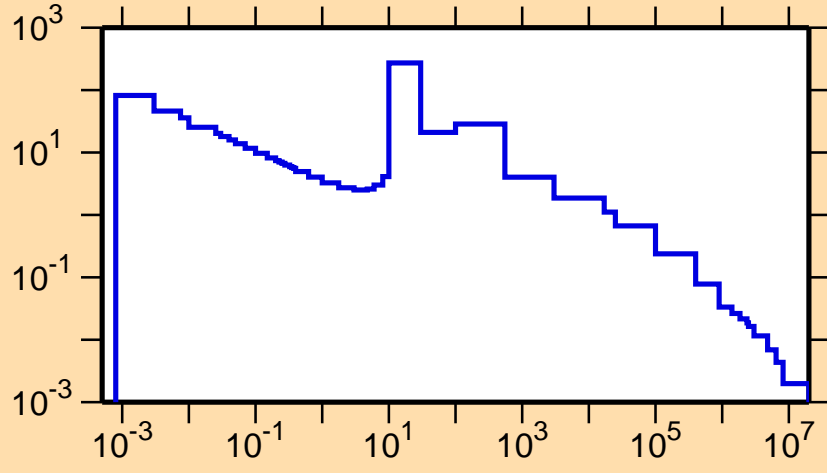
\sigma vs. E for ^{103}\text{Pd}(n,\gamma)
