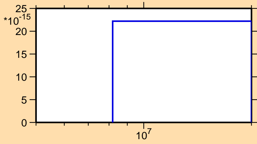
\sigma vs. E for ^{103}\text{Pd}(\text{mt117})
