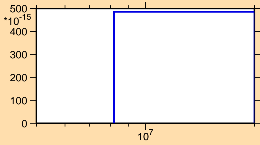
\sigma vs. E for ^{103}\text{Pd}(n,\text{pd})
