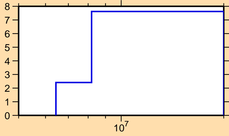
\Delta\sigma/\sigma vs. E for ^{103}\text{Pd}(n,\text{tot.})
