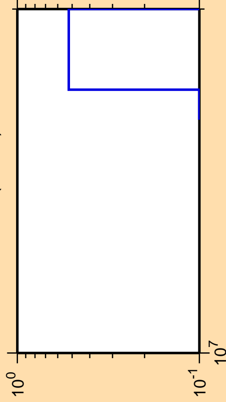
\Delta\sigma/\sigma vs. E for ^{104}\text{Pd}(\text{mt } 45)
