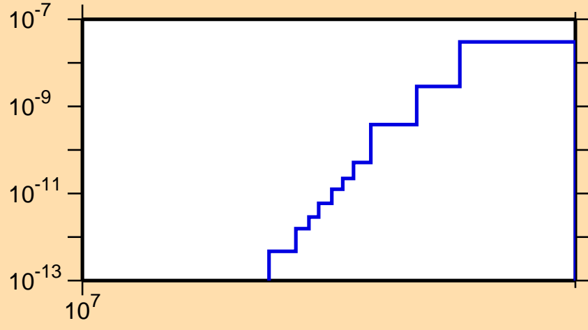
\sigma vs. E for ^{104}\text{Pd}(n,p\alpha)
