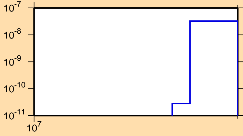
\sigma vs. E for ^{104}\text{Pd}(n,2n\alpha)
