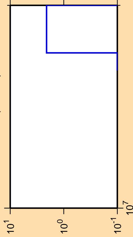
\Delta\sigma/\sigma vs. E for ^{104}\text{Pd}(\text{mt117})
