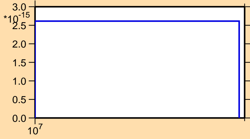
\sigma vs. E for ^{104}\text{Pd}(\text{mt117})
