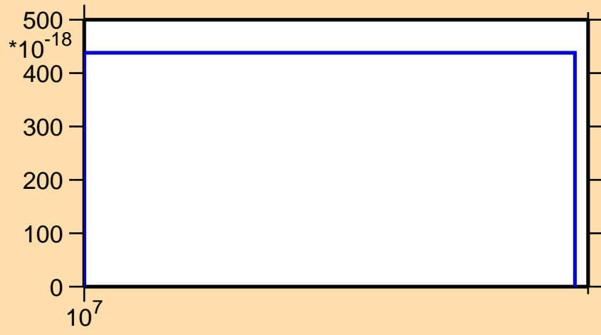
\sigma vs. E for ^{104}\text{Pd}(\text{mt } 45)
