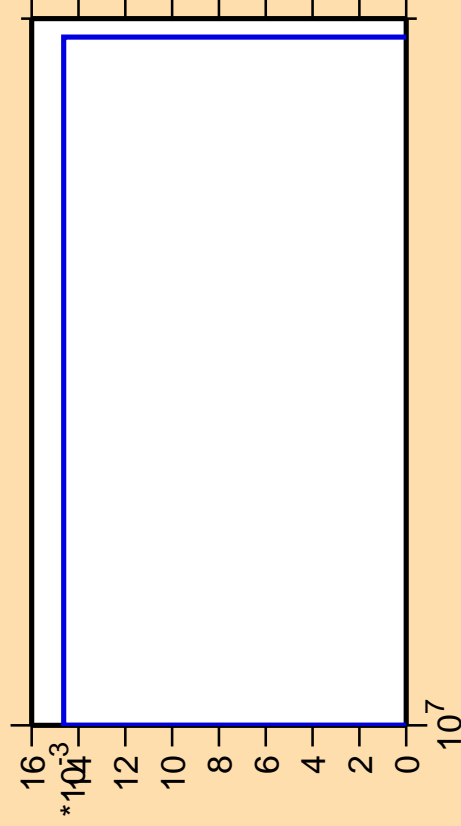
\Delta\sigma/\sigma vs. E for ^{104}\text{Pd}(\text{mt117})
