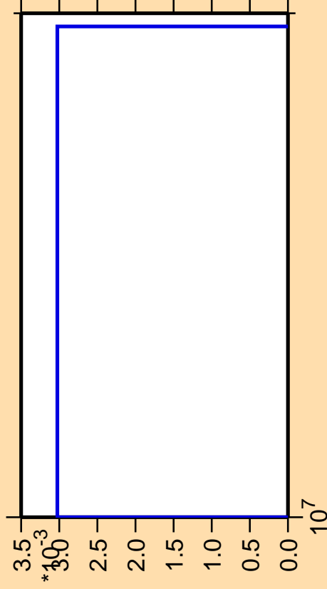
\Delta\sigma/\sigma vs. E for ^{104}\text{Pd}(\text{mt } 45)
