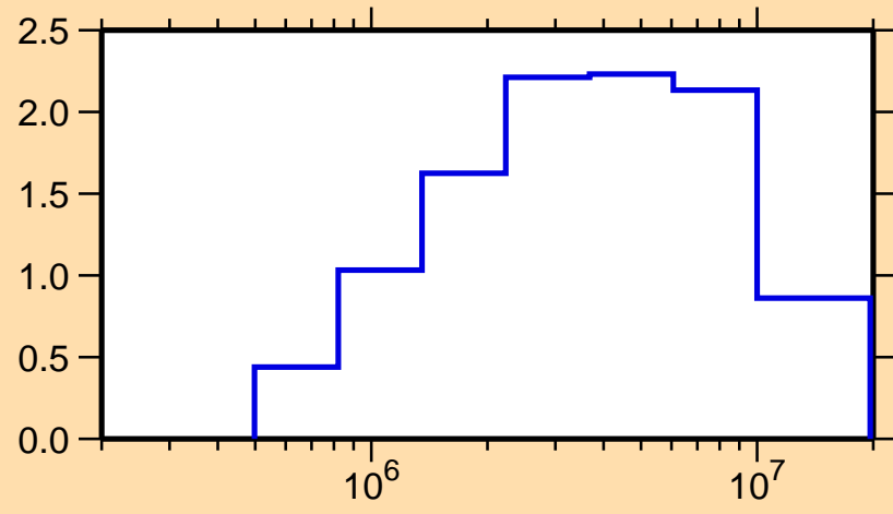
\sigma vs. E for ^{104}\text{Pd}(n,\text{inel.})
