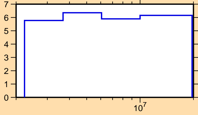
\Delta\sigma/\sigma vs. E for ^{104}\text{Pd}(n,n\text{onel.})
